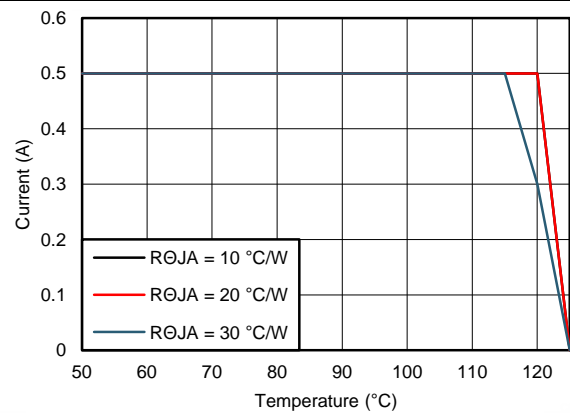
Figure 52. Derating Curve
