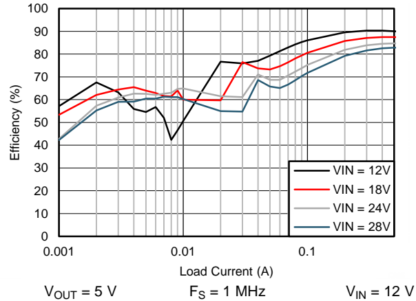
Figure 72. Efficiency
