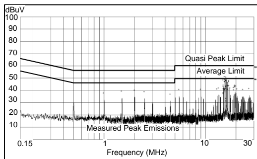
Figure 23. Conducted EMI Curve V_{OUT} = 3.3\text{ V} F_S = 500\text{ kHz} I_{OUT} = 0.5\text{ A} Measured on the LM46000PWPEVM with default BOM. EVM input filter: L_{in} = 1\text{ }\mu\text{H} C_d = 47\text{ }\mu\text{F} C_{IN4} = 68\text{ }\mu\text{F}
