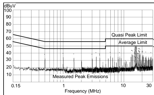
Figure 24. Conducted EMI Curve V_{OUT} = 5\text{ V} F_S = 500\text{ kHz} I_{OUT} = 0.5\text{ A} Measured on the LM46000PWPEVM with L = 44\text{ }\mu\text{H} , C_{OUT} = 66\text{ }\mu\text{F} , C_{FF} = 33\text{ pF} . EVM input filter L_{in} = 1\text{ }\mu\text{H} C_d = 47\text{ }\mu\text{F} C_{IN4} = 68\text{ }\mu\text{F}
