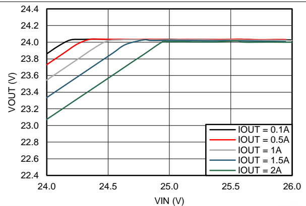
Figure 18. Dropout Curve V_{OUT} = 24\text{ V} F_S = 500\text{ kHz}
