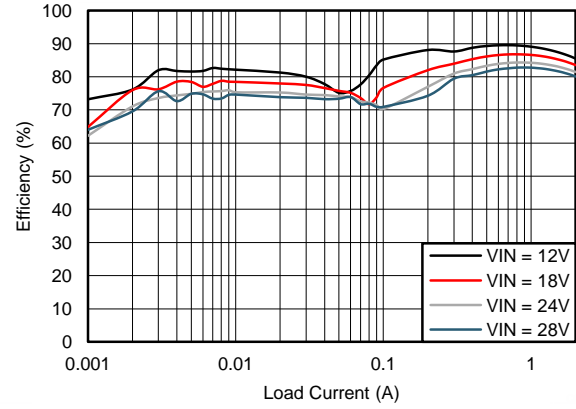
Figure 48. Efficiency
