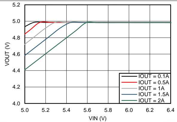
Figure 16. Dropout Curve V_{OUT} = 5\text{ V} F_S = 1\text{ MHz}
