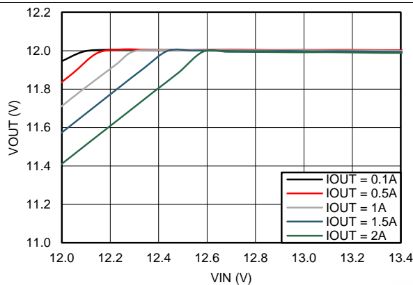
Figure 17. Dropout Curve V_{OUT} = 12\text{ V} F_S = 500\text{ kHz}
