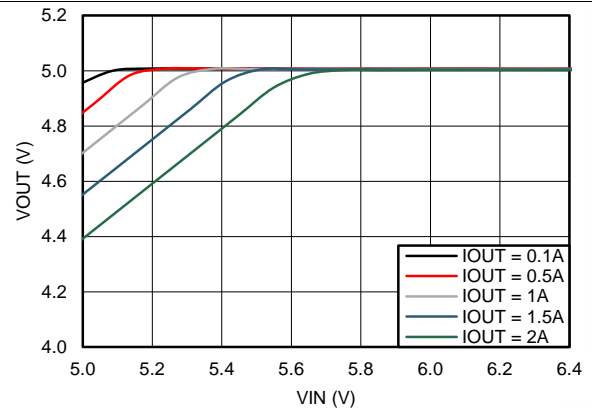
Figure 14. Dropout Curve V_{OUT} = 5\text{ V} F_S = 200\text{ kHz}
