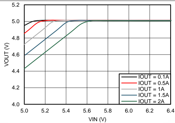
Figure 15. Dropout Curve V_{OUT} = 5\text{ V} F_S = 500\text{ kHz}
