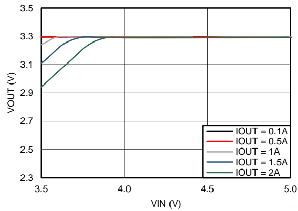
Figure 13. Dropout Curve V_{OUT} = 3.3\text{ V} F_S = 500\text{ kHz}
