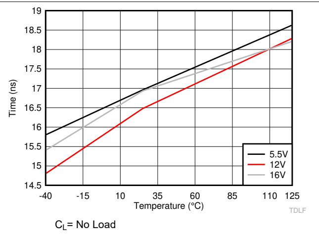
图 6-23. LO Falling Propagation Delay (TDLFF)
