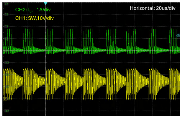
图 8-13. V_{in} = 14.4V , V_{out} = 24V , DEM, I_{load} = 0.1A
