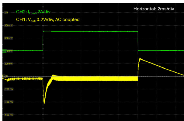
图 8-17. 负载瞬态, V_{in} = 14.4V , V_{out} = 24V , DEM , I_{load} = 0A 至 3.125A , 1A/\mu s
