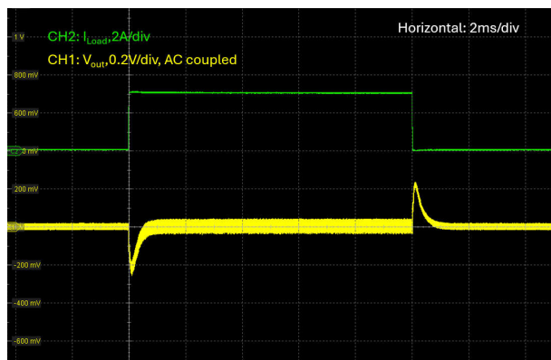
图 8-16. 负载瞬态, V_{in} = 14.4V , V_{out} = 24V , FPWM , I_{load} = 0A 至 3.125A , 1A/\mu s
