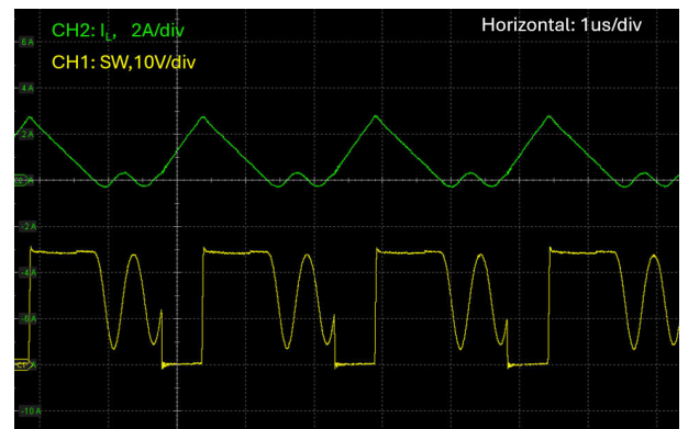
图 8-14. V_{in} = 14.4V , V_{out} = 24V , DEM, I_{load} = 0.5A
