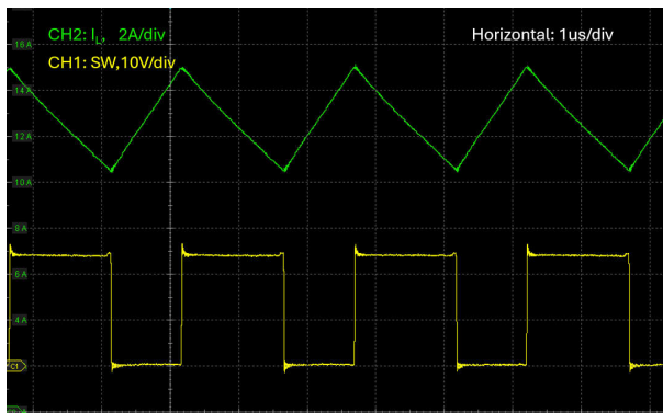
图 8-15. V_{in} = 14.4V , V_{out} = 24V , DEM , I_{load} = 7.5A
