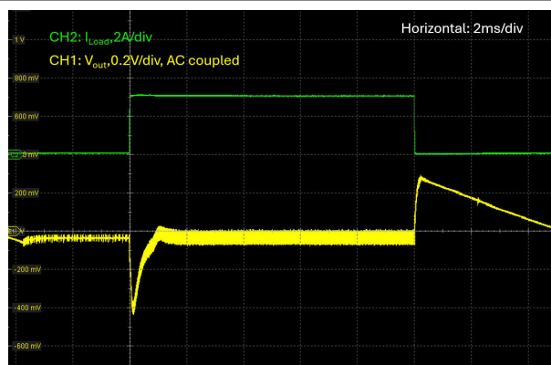
图 7-16. 负载瞬态, V_{in} = 14.4V , V_{out} = 24V , DEM, I_{load} = 0A 至 3.125A , 1A/\mu s
