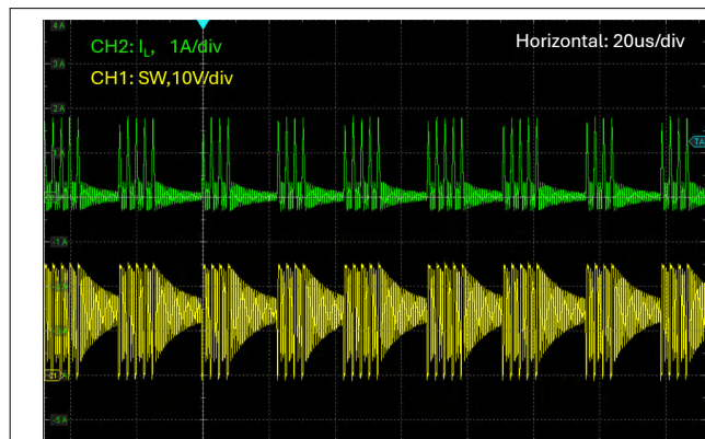
图 7-12. V_{in} = 14.4V , V_{out} = 24V , DEM, I_{load} = 0.1A
