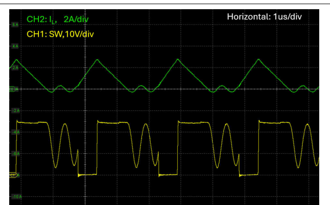
图 7-13. V_{in} = 14.4V , V_{out} = 24V , DEM, I_{load} = 0.5A
