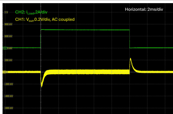
图 7-15. 负载瞬态, V_{in} = 14.4V , V_{out} = 24V , FPWM, I_{load} = 0A 至 3.125A , 1A/\mu s
