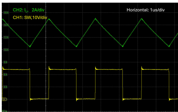
图 7-14. V_{in} = 14.4V , V_{out} = 24V , DEM, I_{load} = 7.5A
