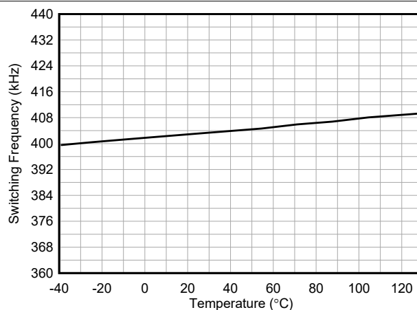
图 6-2. Switching Frequency vs Temperature R_{(RT)} = 75\text{k}\Omega
