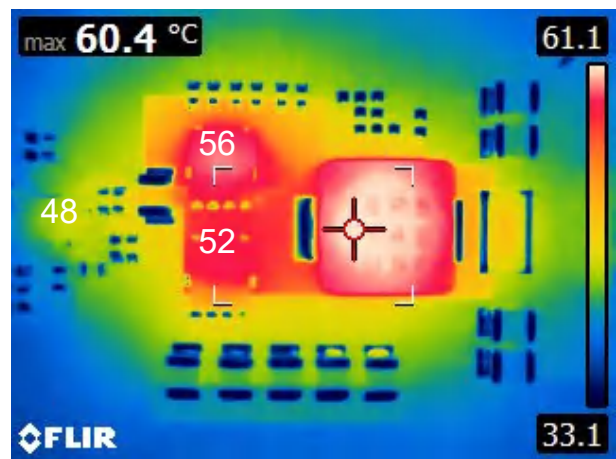
Figure 9-13. V_{SUPPLY} = 48V , I_{LOAD} = 8A , T_A = 25^{\circ}C , No Airflow
