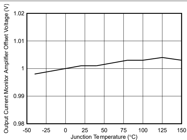
Figure 6-14. IMON Amplifier Voltage Offset vs Temperature
