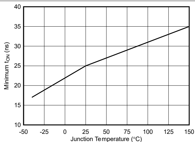
Figure 6-12. Minimum On-Time vs Temperature
