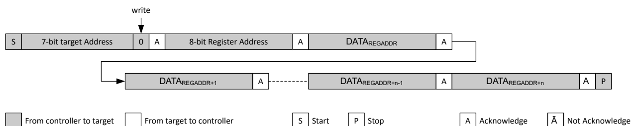
Figure 7-14. Sequential WRITE Starting at a Defined Register Address
