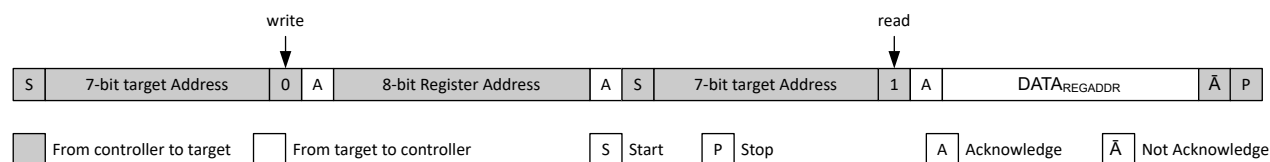
Figure 7-11. Single READ From a Defined Register Address
