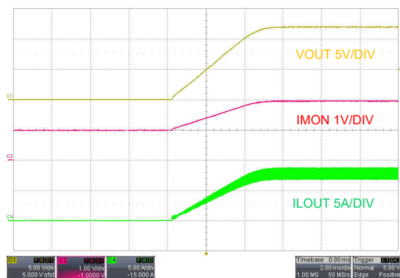
Figure 9-6. Start-Up, EN ON, V_{SUPPLY} = 48V , I_{LOAD} = 8A Resistive Load
