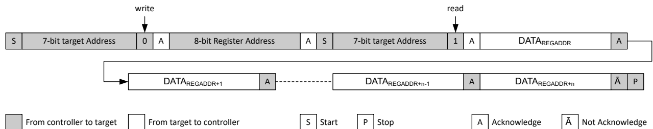
Figure 7-12. Sequential READ Starting from a Defined Register Address
