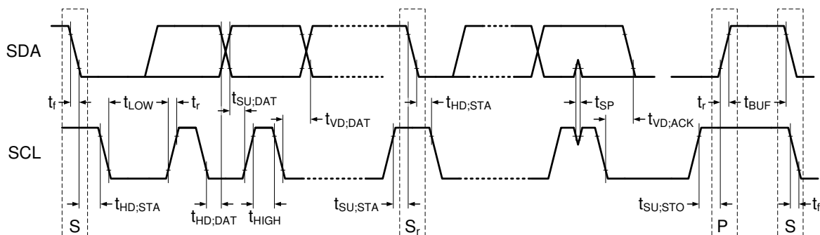
Figure 7-9. I 2 C Data Transmission Timing
