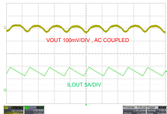
Figure 9-8. Output Ripple, V_{SUPPLY} = 48V , I_{LOAD} = 8A
