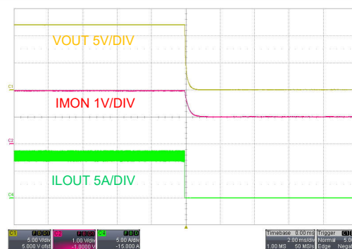
Figure 9-7. Shutdown, EN OFF, V_{SUPPLY} = 48V , I_{LOAD} = 8A Resistive Load
