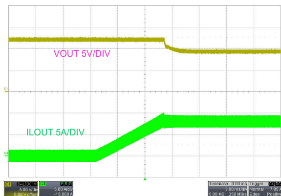
Figure 9-12. CV to CC Mode Transition, V_{SUPPLY} = 48V , V_{LOAD} = 12V to 9V
