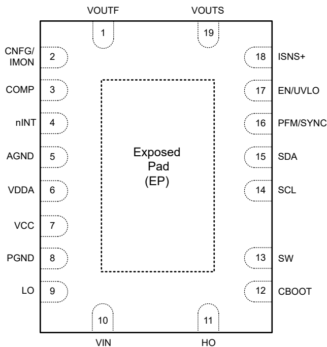
Figure 5-1. RGY 19-Pin VQFN (Top View)
