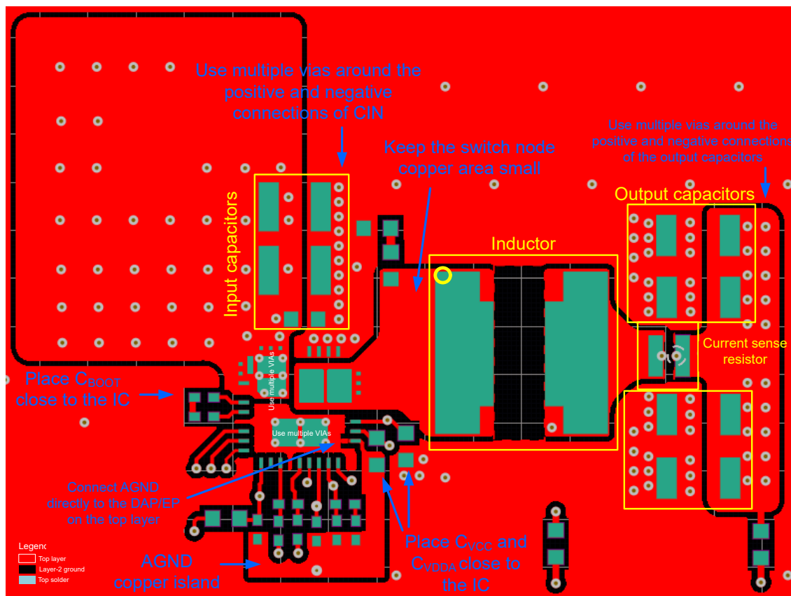
Figure 9-15. PCB Top Layer
