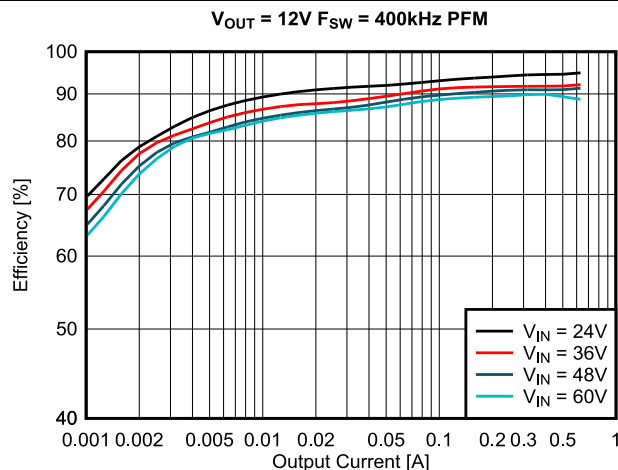
Figure 9-5. PFM Mode Efficiency, Log Scale
