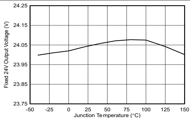
Figure 6-8. Fixed Output Voltage vs Temperature, V_{OUT} = 24V
