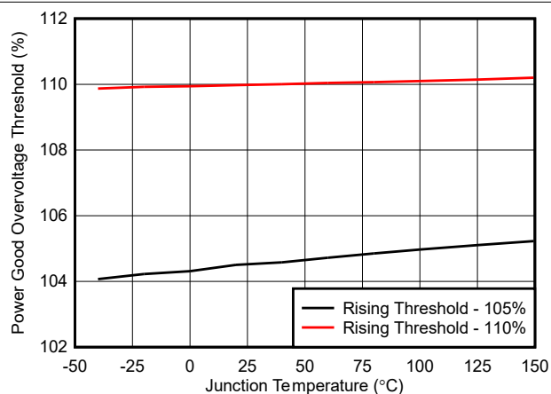
Figure 6-10. PG Overvoltage Threshold vs Temperature
