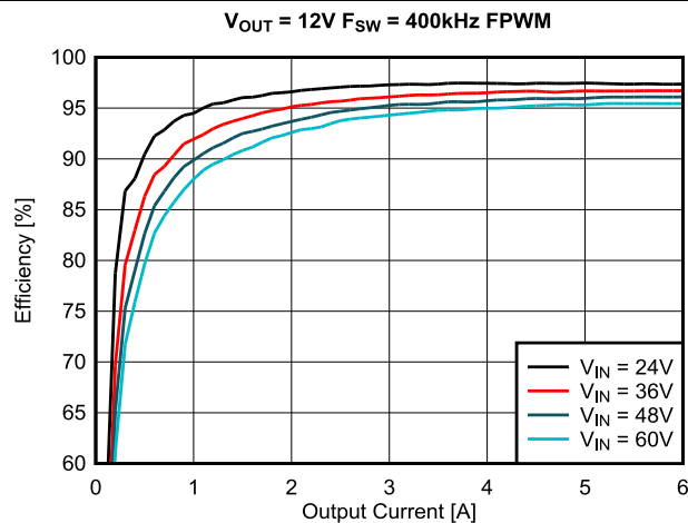
Figure 9-4. FPWM Mode Efficiency, Linear Scale
