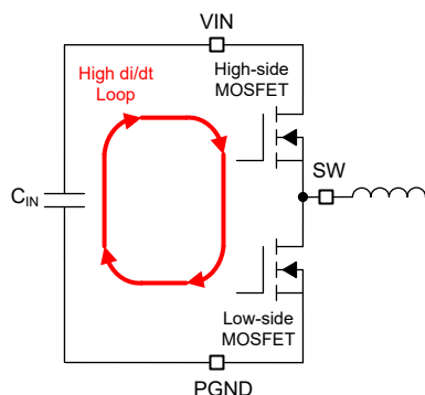
Figure 9-14. Input Current Loop
