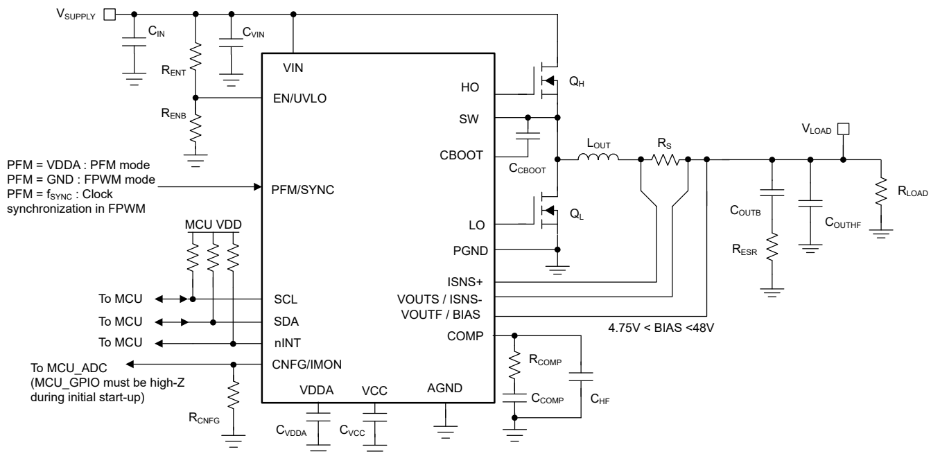
Figure 9-3. Application Circuit With I 2 C Interface
