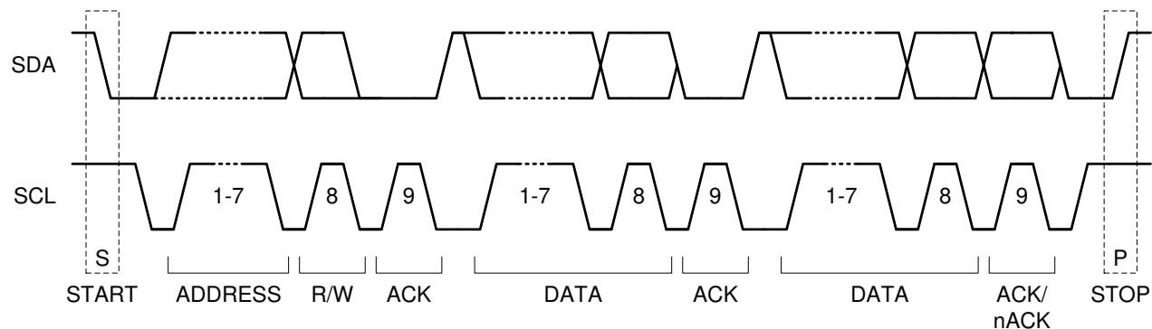
Figure 7-8. I 2 C START / STOP / ACKNOWLEDGE Protocol
