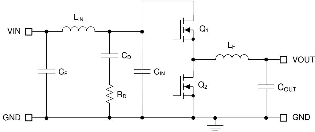
Figure 9-2. Buck Regulator With π-Stage EMI Filter
