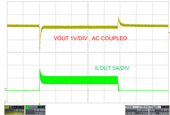
Figure 9-11. Load Transient Response, V_{SUPPLY} = 48V , PFM, 0A to 4A
