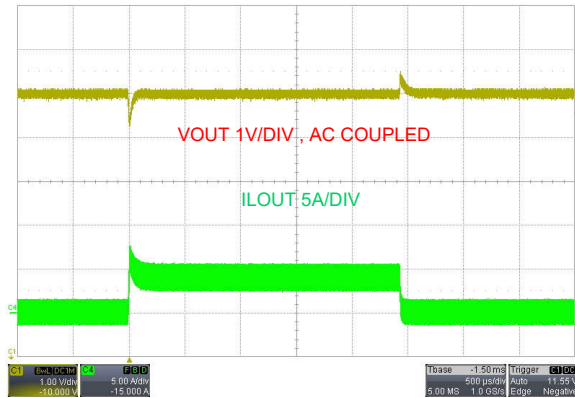
Figure 9-10. Load Transient Response, V_{SUPPLY} = 48V , FPWM, 0A to 4A
