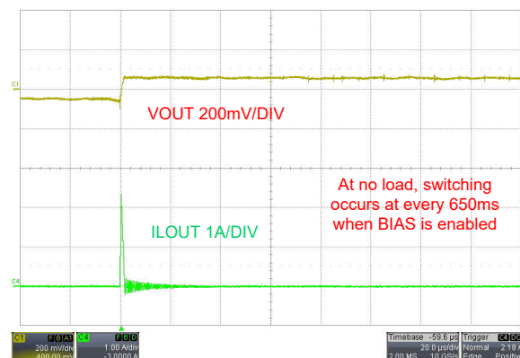
Figure 9-9. No Load Operation in PFM Mode, V_{SUPPLY} = 48V , I_{LOAD} = 0A
