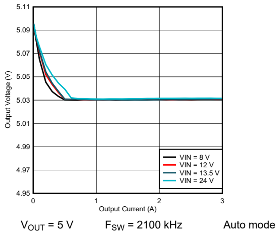
图 9-18. LM61430-Q1 Load and Line Regulation
