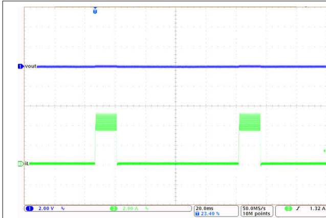
图 8-12. Inductor Current Bursts During Hiccup
