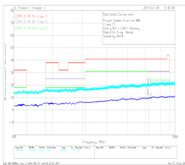
V_{OUT} = 5\text{ V} F_{SW} = 400\text{ kHz} I_{OUT} = 5\text{ A} Frequency tested: 300 MHz to 1 GHz Tested on 6-A variant with LM61460EVM
