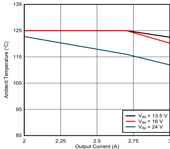
图 9-2. Maximum Ambient Temperature versus Output Current
