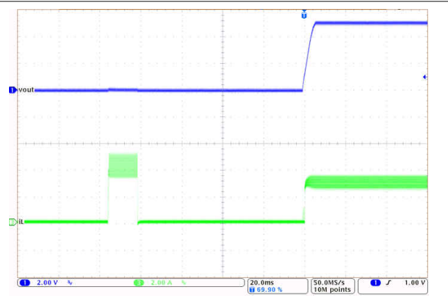
图 8-13. Short-Circuit Recovery
