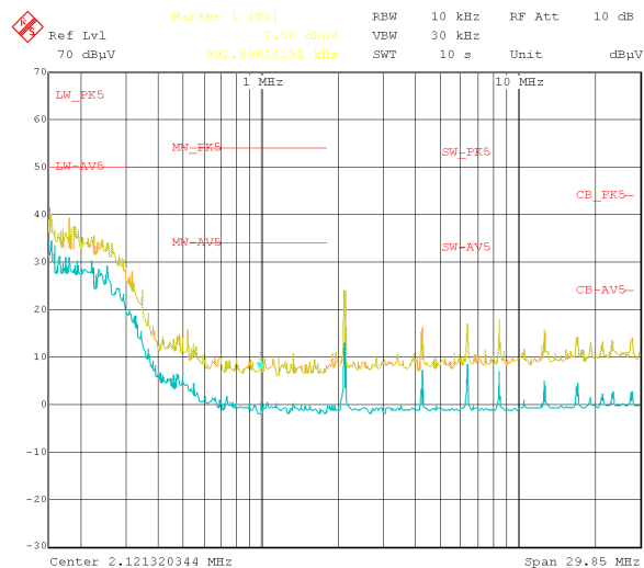
F_{SW} = 2100\text{ kHz} V_{OUT} = 5\text{ V} I_{OUT} = 5\text{ A} Frequency tested: 150 kHz to 30 MHz Tested on 6-A variant with LM61460EVM
