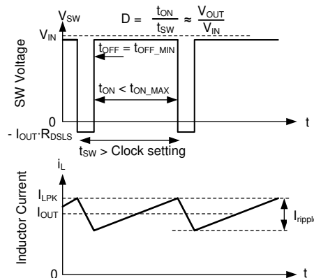
图 8-19. Frequency and Output Voltage in Dropout
