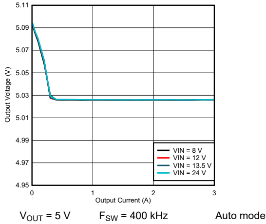
图 9-16. LM61430-Q1 Load and Line Regulation
