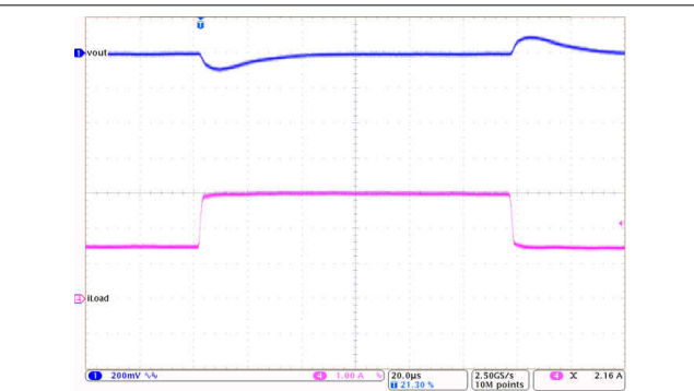
V_{OUT} = 5\text{ V} F_{SW} = 2100\text{ kHz} FPWM mode I_{OUT} = 1.5\text{ A to }3\text{ A} V_{IN} = 13.5\text{ V} T_R = T_F = 6\text{ }\mu\text{s} to 0 A
