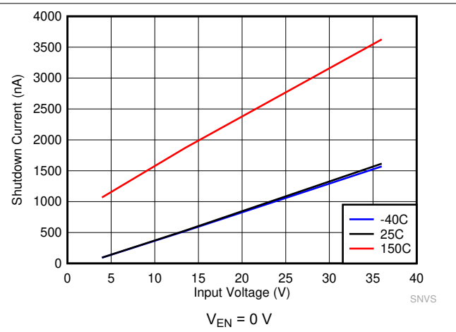
图 8-2. Shutdown Supply Current
