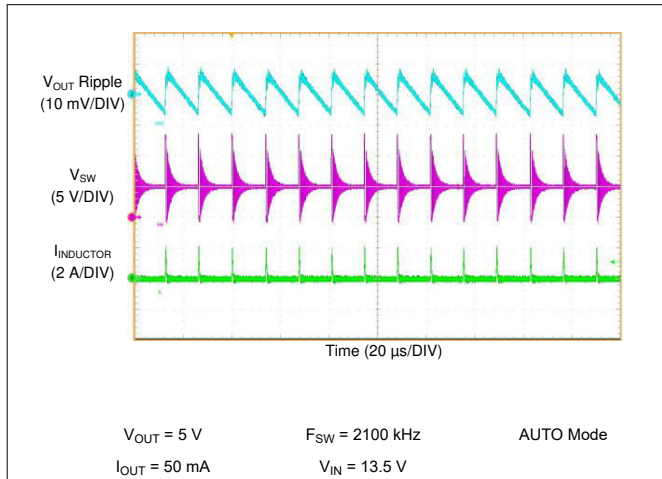
图 10-29. LM61460-Q1 Switching Waveform and V_{OUT} Ripple
