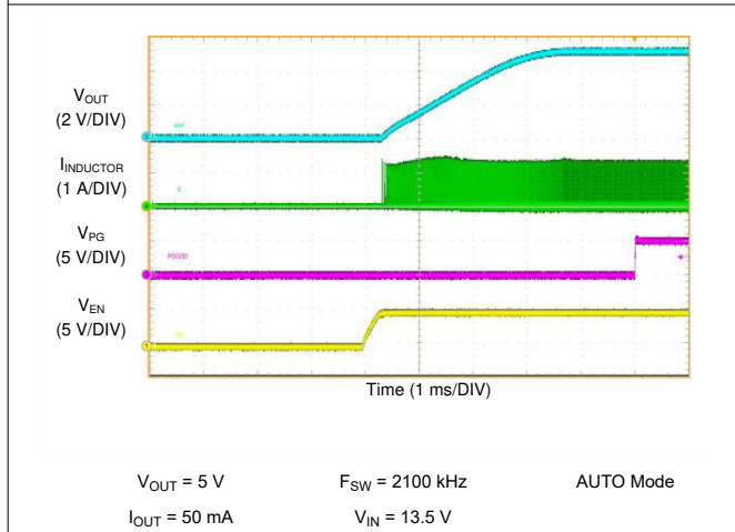
图 10-31. LM61460-Q1 Start-up with 50-mA Load
