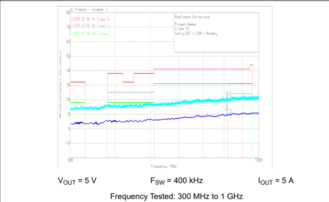
图 10-52. Radiated EMI Log Horizontal versus CISPR25 Limits
