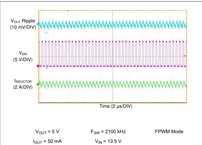
图 10-30. LM61460-Q1 Switching Waveform and V_{OUT} Ripple
