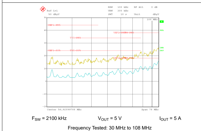
图 10-55. Conducted EMI versus CISPR25 Limits (Yellow: Peak Signal, Blue: Average Signal)
