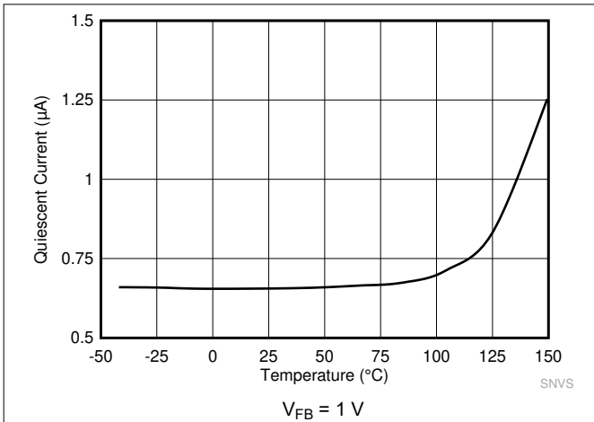
图 8-1. Non-Switching Input Supply Current
