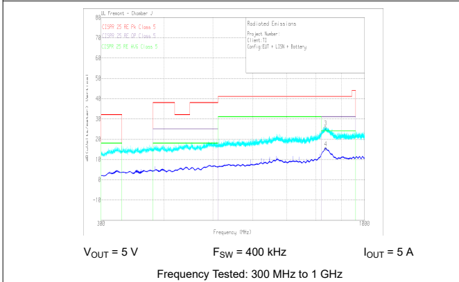
图 10-51. Radiated EMI Log Vertical versus CISPR25 Limits
