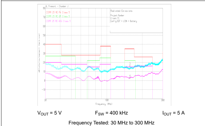
图 10-49. Radiated EMI Bicon Vertical versus CISPR25 Limits
