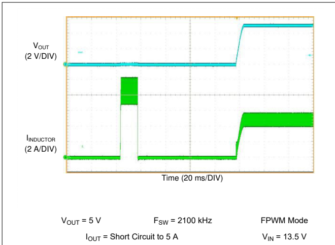
图 10-35. LM61460-Q1 Short Circuit Recovery
