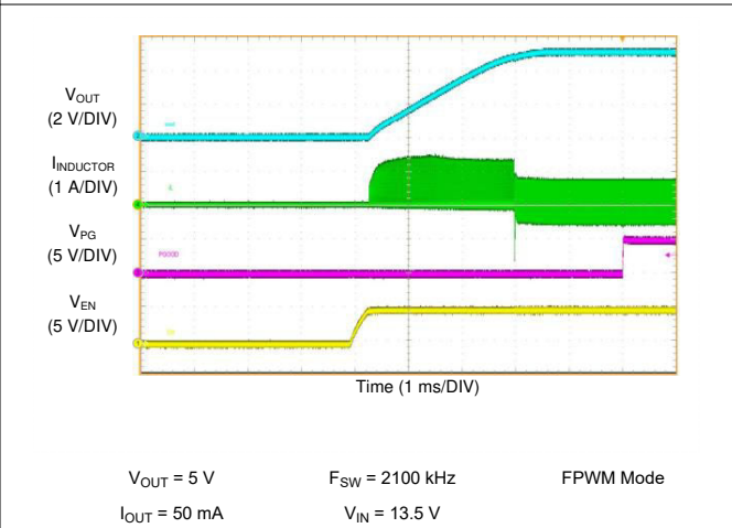
图 10-32. LM61460-Q1 Start-up with 50-mA
