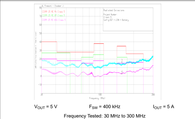
图 10-50. Radiated EMI Bicon Horizontal versus CISPR25 Limits
