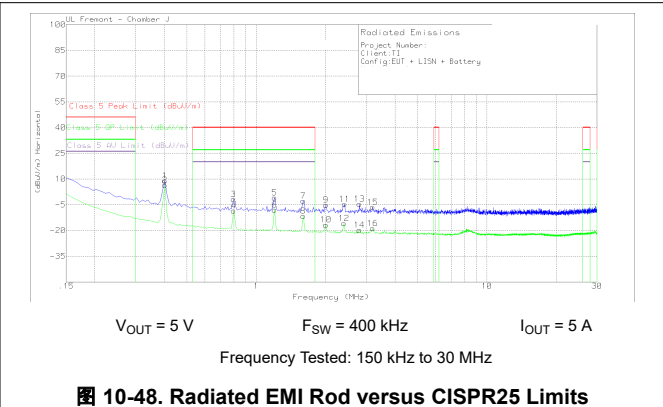
图 10-48. Radiated EMI Rod versus CISPR25 Limits
