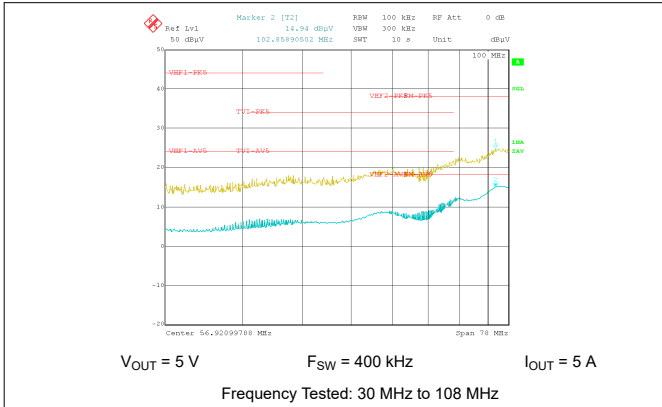
图 10-47. Conducted EMI versus CISPR25 Limits (Yellow: Peak Signal, Blue: Average Signal)
