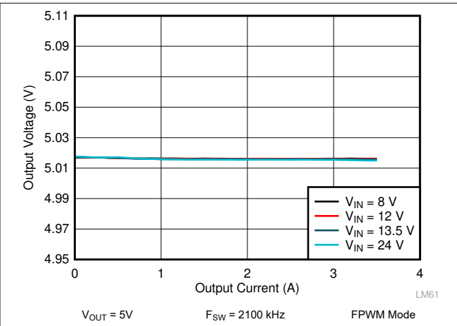
图 9-12. LM62435-Q1 Load and Line Regulation
