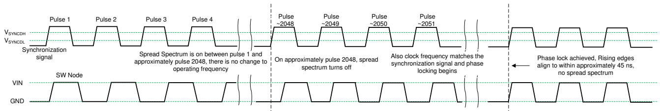
图 8-12. Synchronization Process
