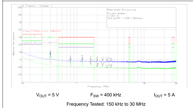
图 9-27. Radiated EMI Rod versus CISPR25 Limits
