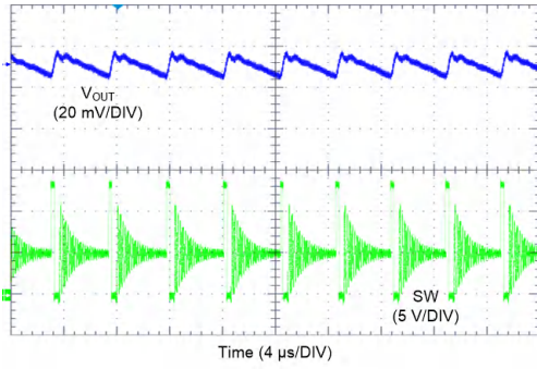
图 10-17. LM62440-Q1 Switching Waveform and V_{OUT} Ripple
