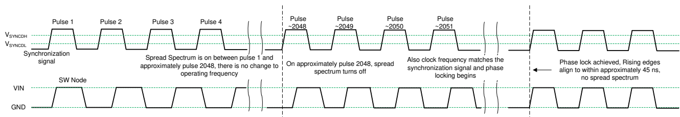
图 9-12. Synchronization Process
