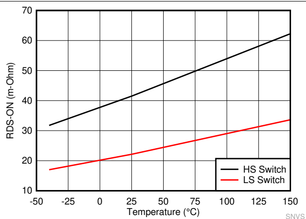
图 8-6. High-Side and Low-Side Switches R_{DS\_ON}
