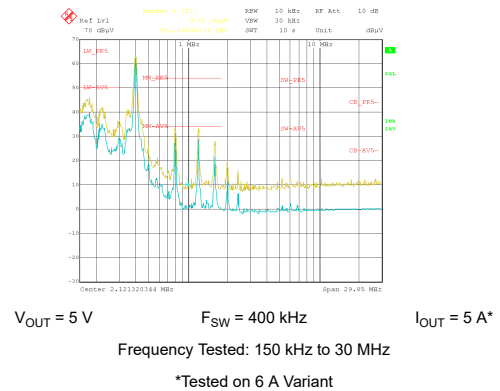
图 10-26. Conducted EMI versus CISPR25 Limits (Yellow: Peak Signal, Blue: Average Signal), LM61460EVM
