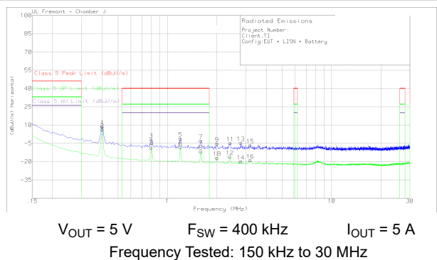
图 10-28. Radiated EMI Rod versus CISPR25 Limits, LM61460EVM
