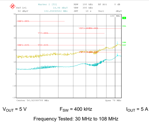
图 10-27. Conducted EMI versus CISPR25 Limits (Yellow: Peak Signal, Blue: Average Signal), LM61460EVM
