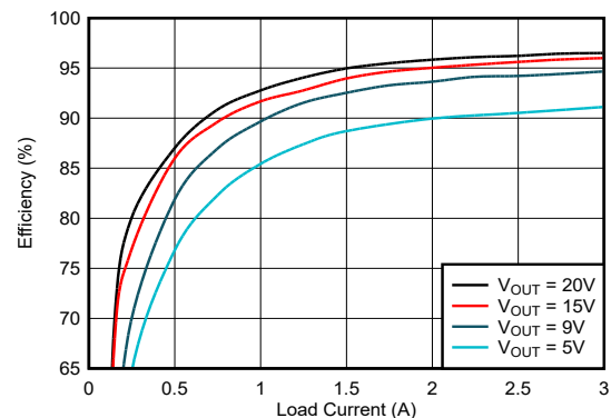
典型效率，V IN = 48V，f SW = 400kHz
