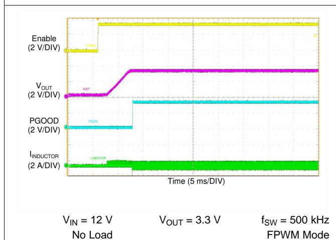
图 63. LM76003 Start-up Waveform
