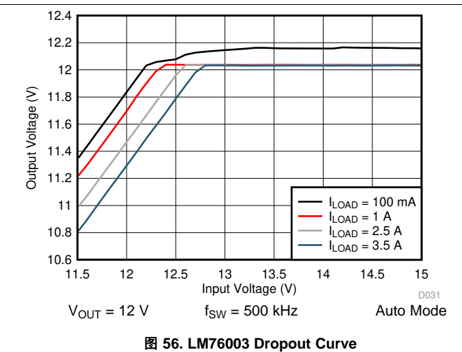
图 56. LM76003 Dropout Curve
