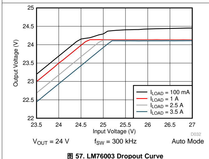
图 57. LM76003 Dropout Curve
