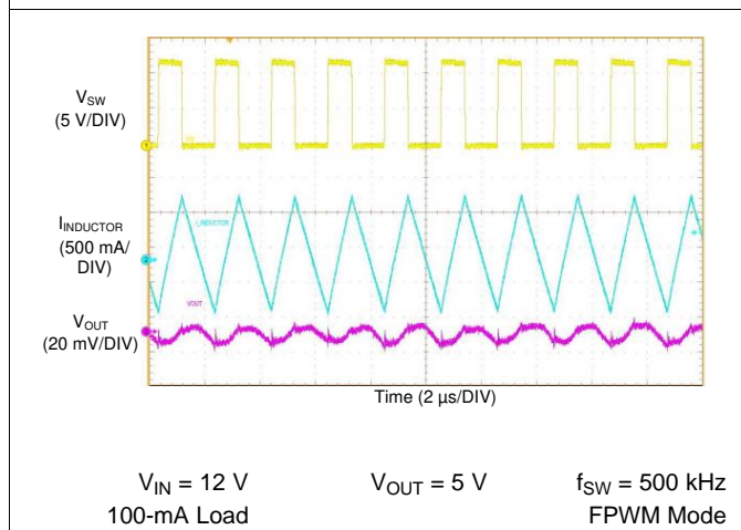
图 61. LM76003 Switching Waveform and Output Ripple
