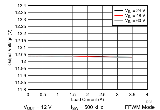
图 46. LM76003 Load and Line Regulation
