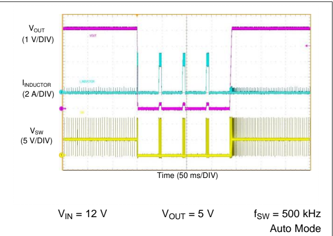
图 72. LM76003 Short-Circuit Behavior With Hiccup
