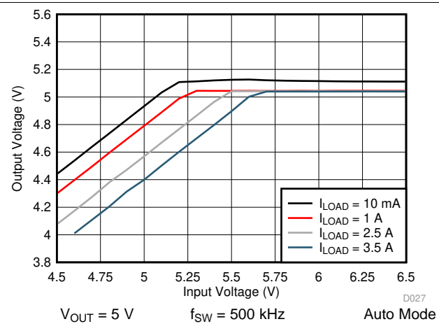
图 52. LM76003 Dropout Curve
