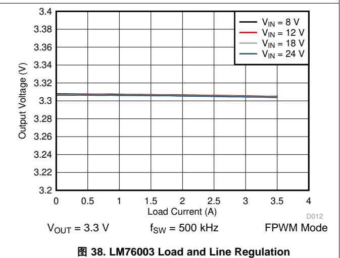
图 38. LM76003 Load and Line Regulation
