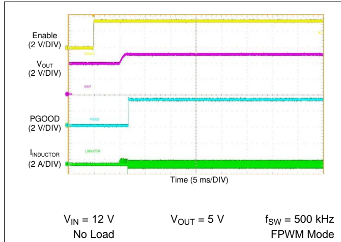
图 71. LM76002 Start-up With Pre-Biased Output
