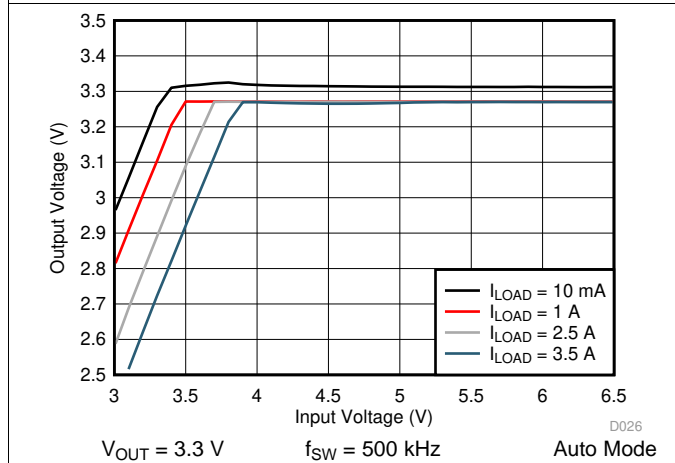
图 51. LM76003 Dropout Curve
