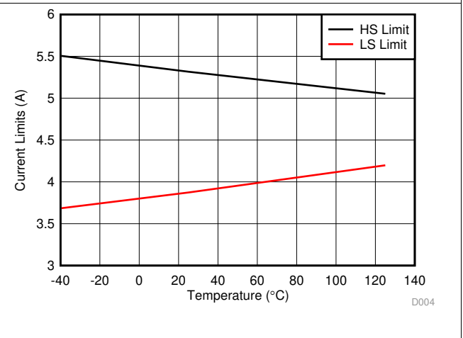
图 4. LM76003 High-Side and Low-Side Current Limits
