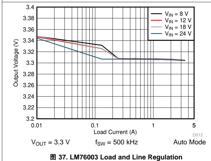
图 37. LM76003 Load and Line Regulation
