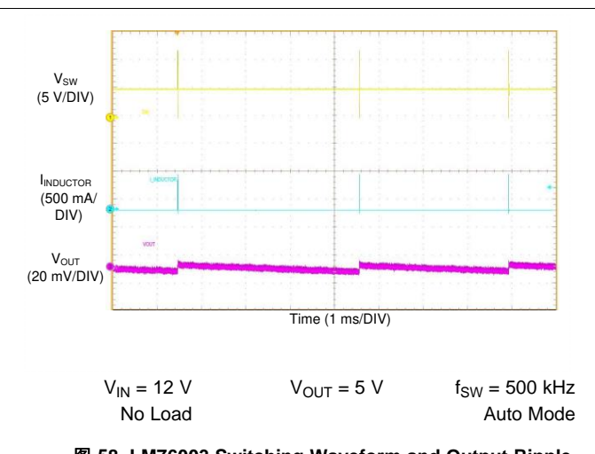
图 58. LM76003 Switching Waveform and Output Ripple
