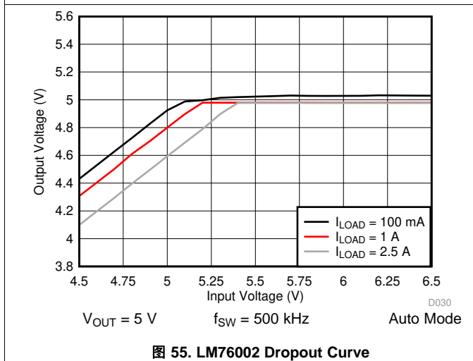
图 55. LM76002 Dropout Curve
