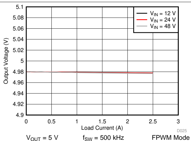
图 50. LM76002 Load and Line Regulation
