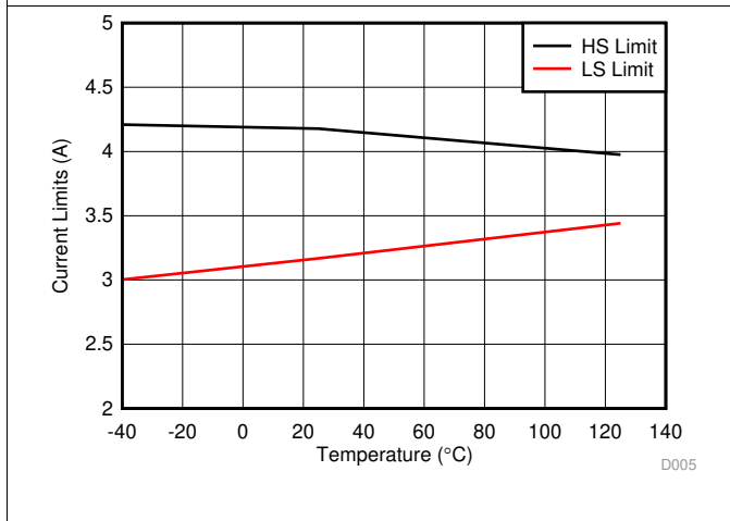
图 5. LM76002 High-Side and Low-Side Current Limits
