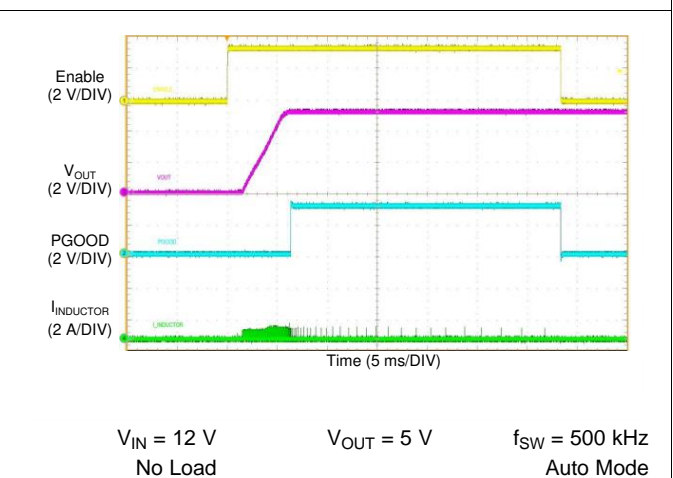
图 64. LM76003 Start-up Waveform
