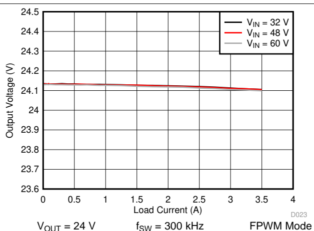
图 48. LM76003 Load and Line Regulation
