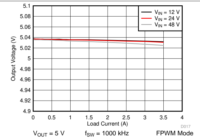
图 42. LM76003 Load and Line Regulation
