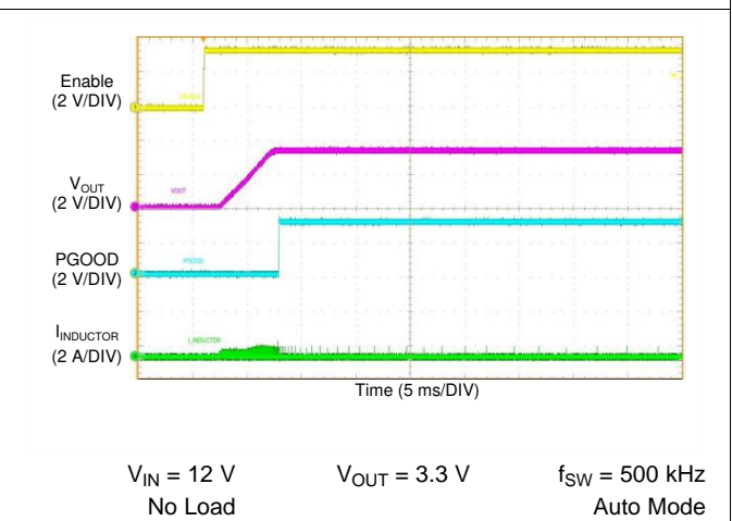
图 62. LM76003 Start-up Waveform
