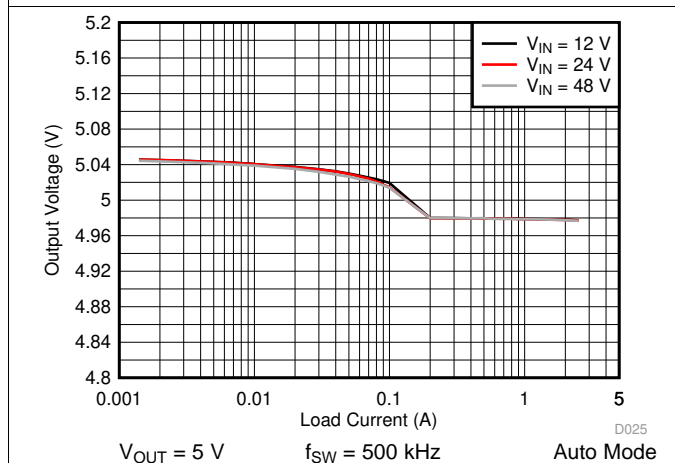
图 49. LM76002 Load and Line Regulation
