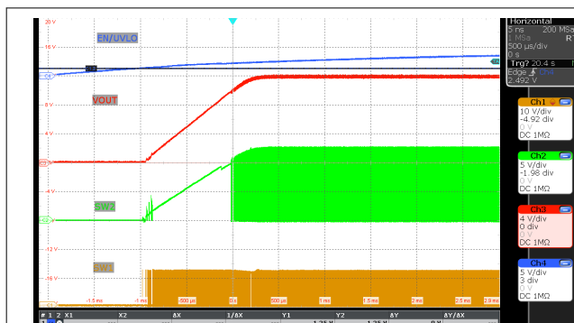
图 10-14. 器件启动 ( V_{(VIN)} = 12V , V_{(VOUT)} = 12V , I_O = 5A , MODE = VCC2 )
