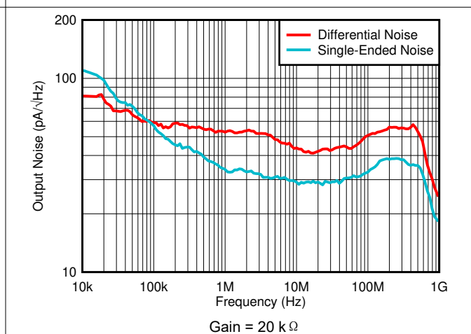
图 6-18. Output Noise Density vs Output Configuration
