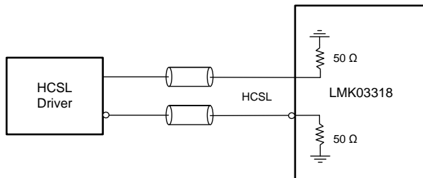
Figure 51. DC-Coupling LMK03318 Inputs With HCSL Signal
