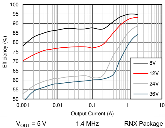
图 8-13. Efficiency
