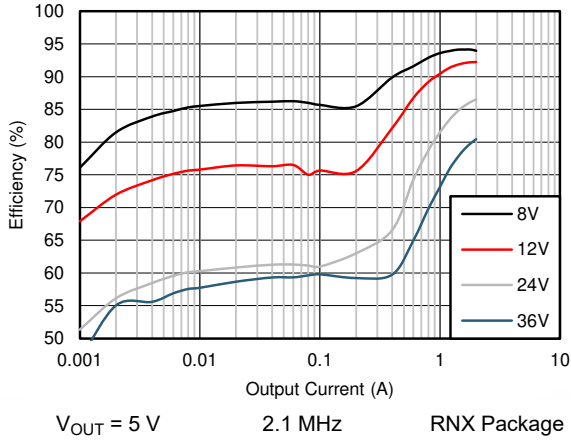
图 8-15. Efficiency
