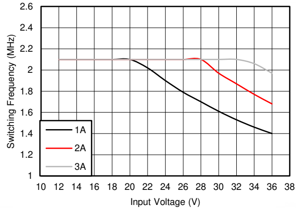
图 7-13. Switching Frequency versus Input Voltage V_{OUT} = 3.3 V
