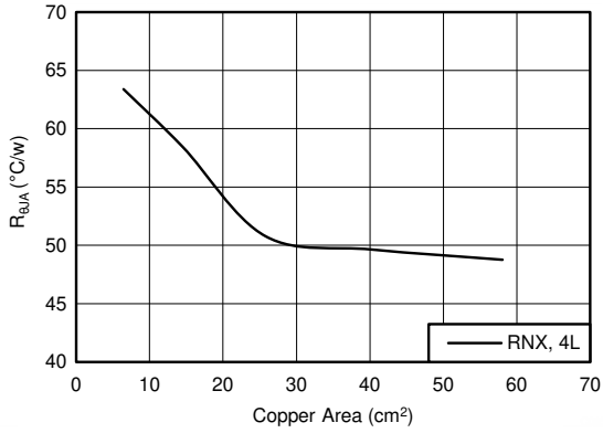
图 8-3. R θJA versus Copper Board Area for the VQFN (RNX) Package
