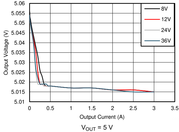
图 8-11. Line and Load Regulation
