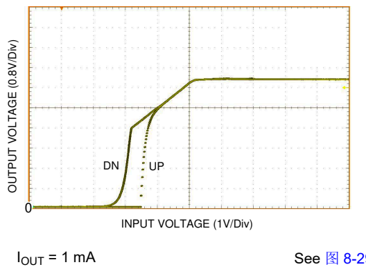
图 6-5. UVLO Thresholds
