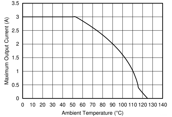
图 8-4. Maximum Output Current versus Ambient Temperature
