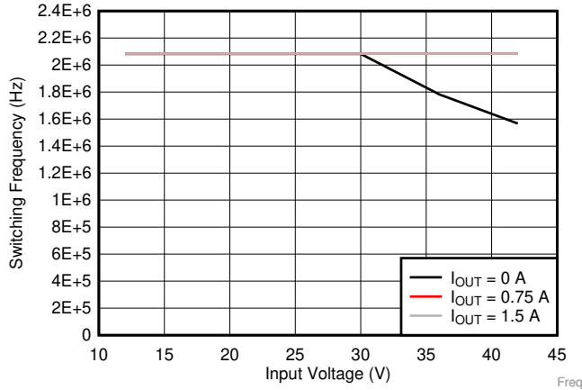
图 8-11. Switching Frequency vs Input Voltage V OUT = 5 V
