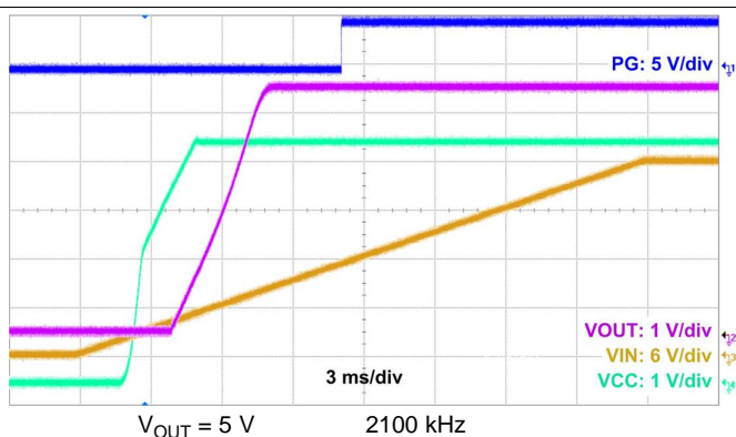
图 50. Start-Up Waveform
