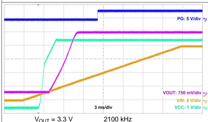
图 51. Start-Up Waveform
