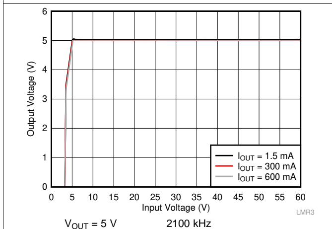
图 47. Line Regulation
