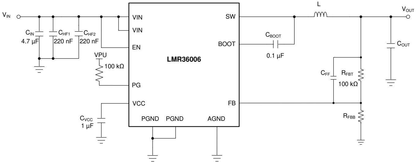
图 18. Example Applications Circuit
