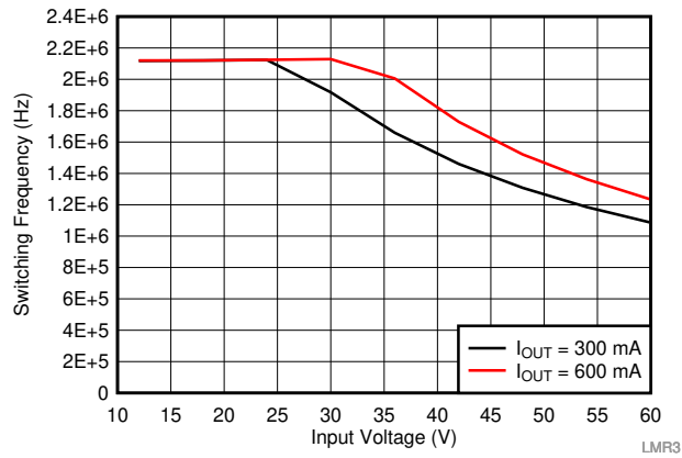
图 17. Switching Frequency vs Input Voltage V OUT = 3.3 V
