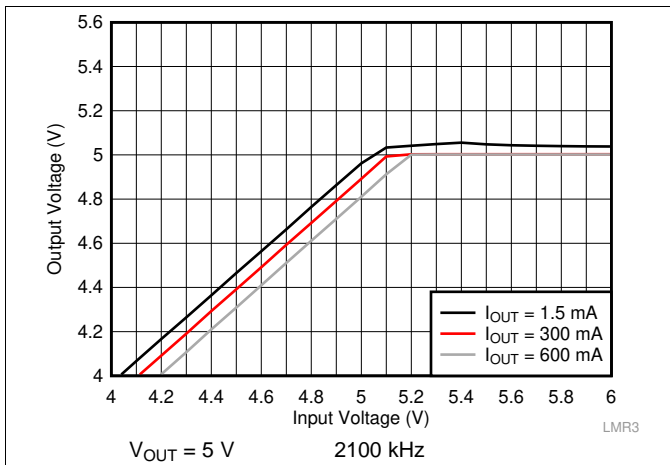
图 49. Overall Dropout Characteristic
