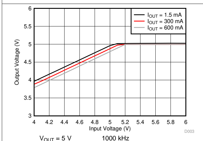
图 25. Overall Dropout Characteristic
