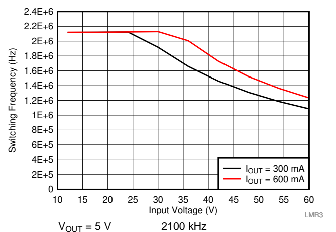
图 48. Switching Frequency vs Input Voltage
