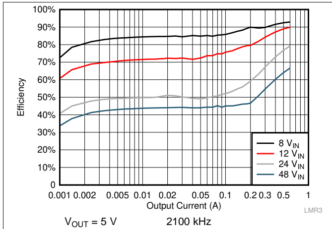
图 43. Efficiency
