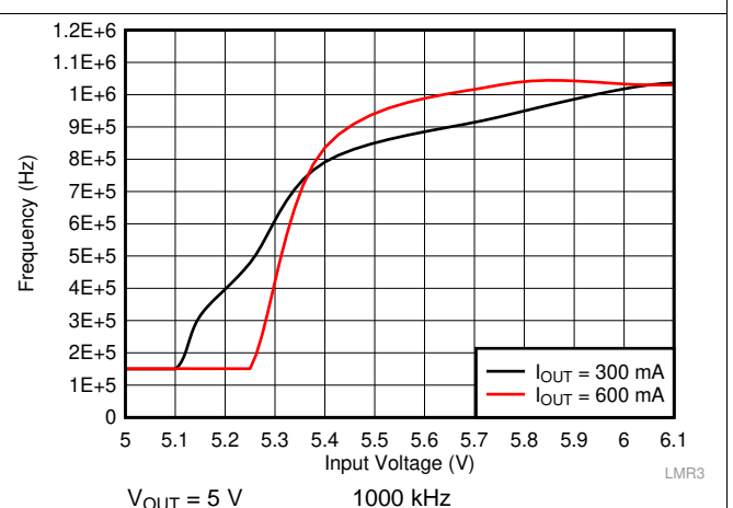
图 26. Frequency Dropout Characteristic
