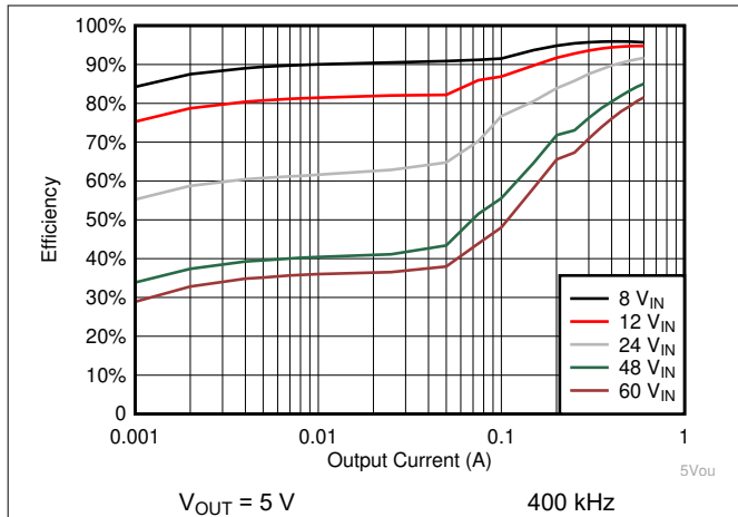
图 9-5. Efficiency
