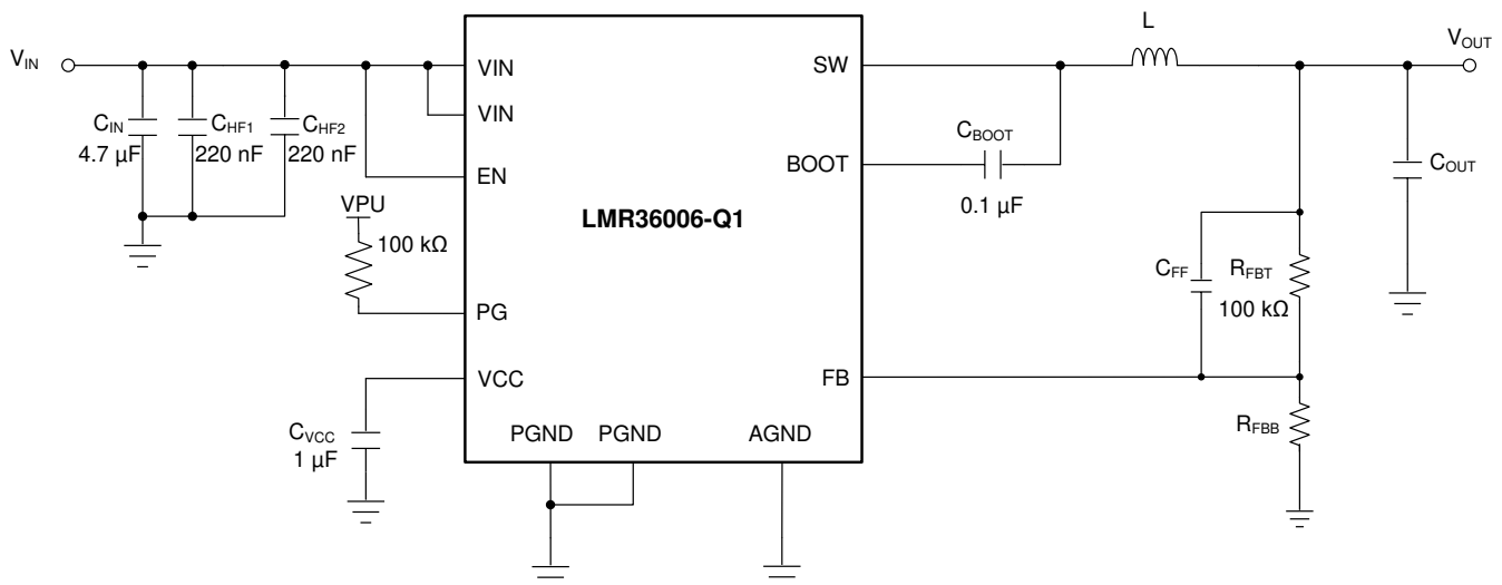
图 9-1. Example Applications Circuit (Adjustable Output)
