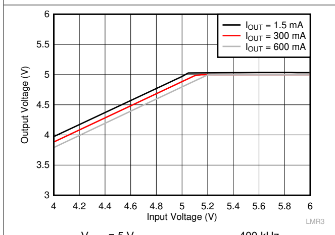
图 9-9. Overall Dropout Characteristic
