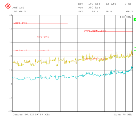
图 9-18. Conducted EMI vs. CISPR25 Limits (Yellow: Peak Signal, Blue: Average Signal)
