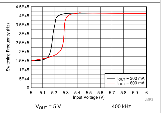
图 9-10. Frequency Dropout Characteristic
