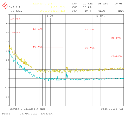
图 9-17. Conducted EMI vs. CISPR25 Limits (Yellow: Peak Signal, Blue: Average Signal)
