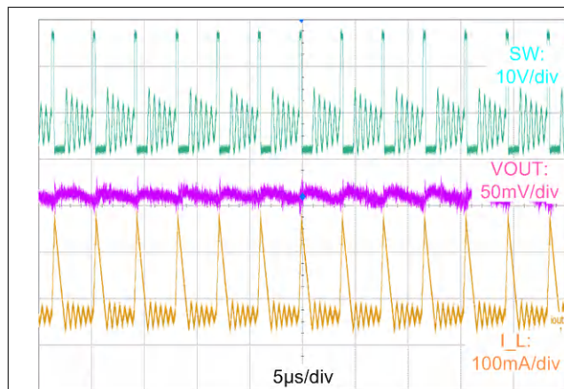
图 8-7. Typical PFM Switching Waveforms V_{IN} = 24 V, V_{OUT} = 5 V, I_{OUT} = 30 mA
