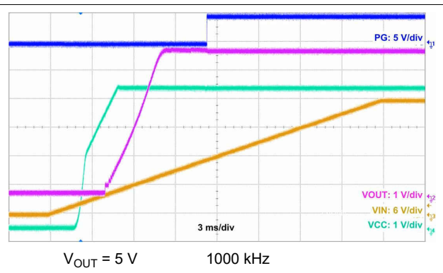
图 10-33. Start-Up Waveform
