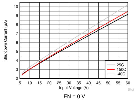
图 8-2. Shutdown Supply Current
