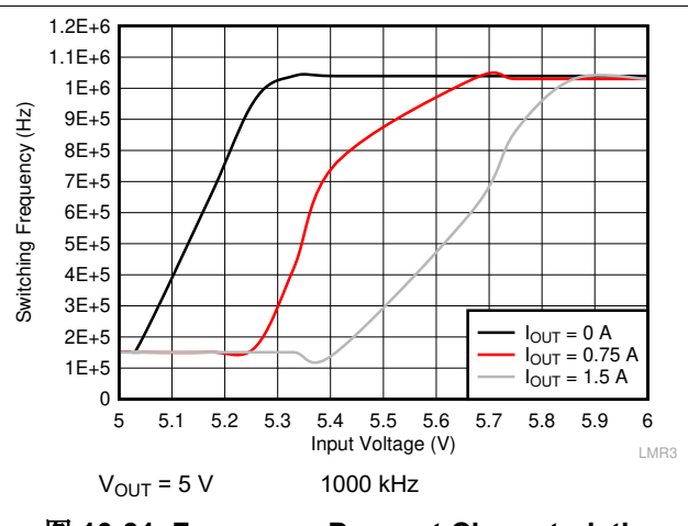
图 10-31. Frequency Dropout Characteristic
