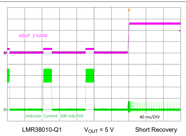
图 8-8. Short-Circuit Recovery
