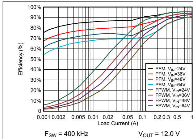
图 6-1. Efficiency vs Load Current
