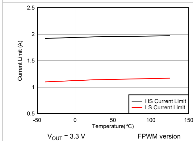
图 6-5. High-Side and Low-Side Current Limit vs Temperature
