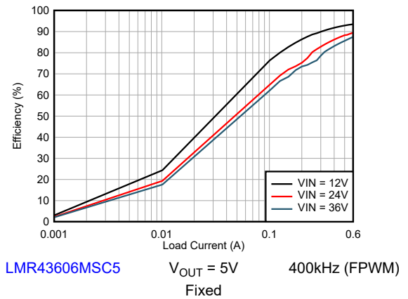
Figure 8-10. Efficiency
