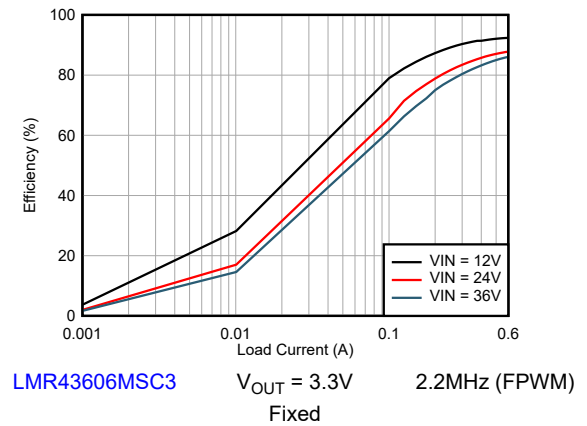
Figure 8-4. Efficiency
