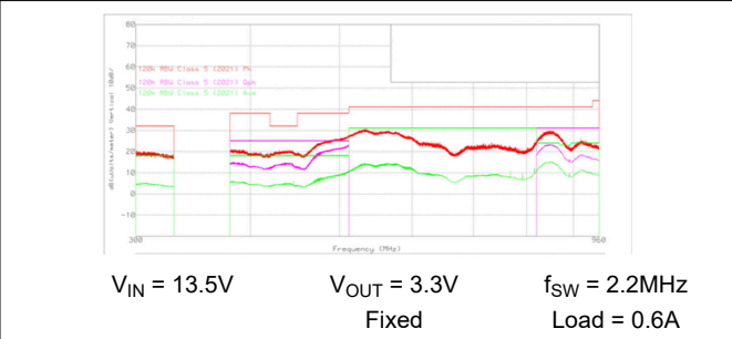
Figure 8-24. Typical CISPR 25 Radiated EMI 300MHz – 1GHz Vertical Log Antenna Red: Peak Detect, Green: Average Detect
