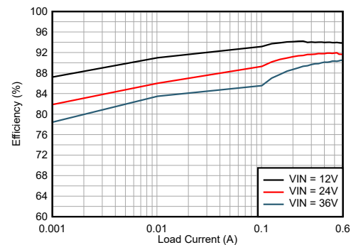
Efficiency: V OUT = 5V (Fixed), 400kHz
