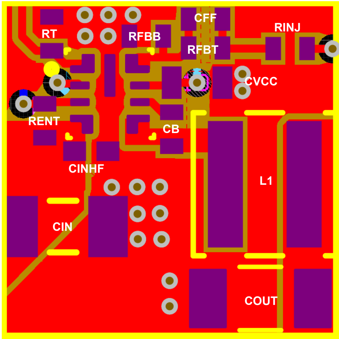
Figure 8-29. Example Layout
