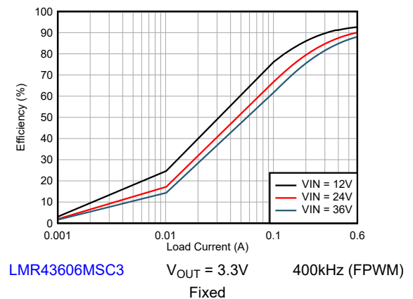
Figure 8-8. Efficiency
