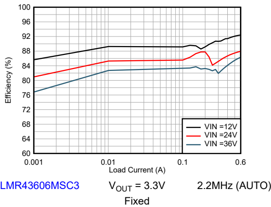
Figure 8-3. Efficiency
