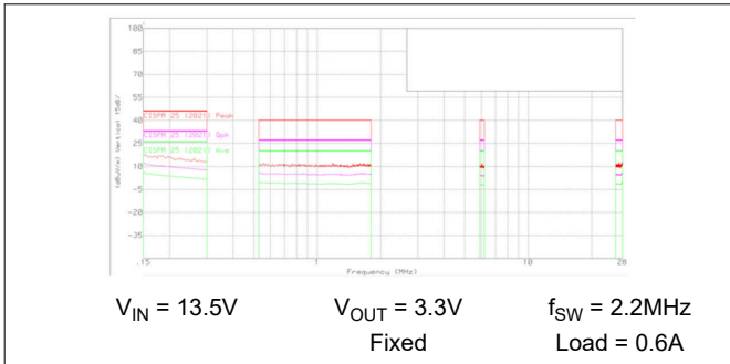
Figure 8-21. Typical CISPR 25 Radiated EMI 150kHz – 30MHz Rod Antenna Red: Peak Detect, Green: Average Detect
