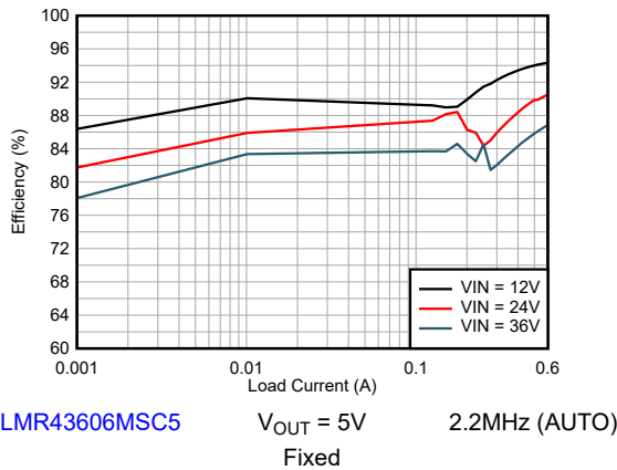
Figure 8-5. Efficiency
