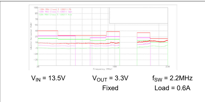
Figure 8-22. Typical CISPR 25 Radiated EMI 30MHz – 230MHz Vertical Bicon Antenna Red: Peak Detect, Green: Average Detect
