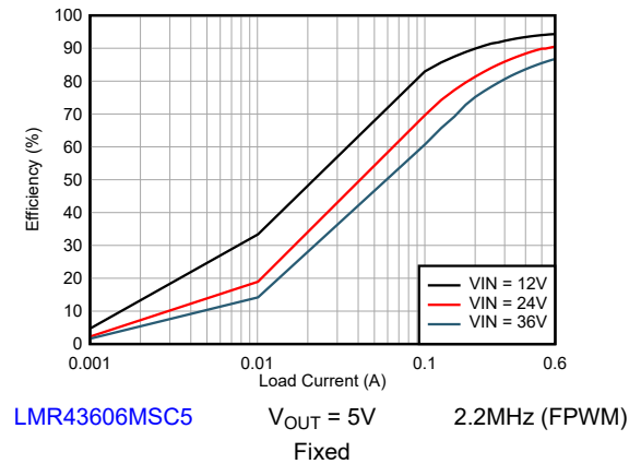
Figure 8-6. Efficiency
