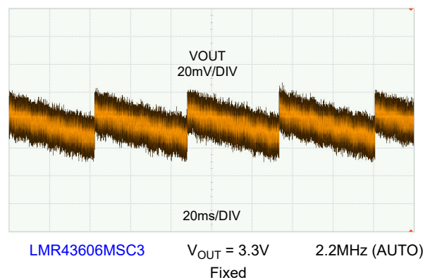
Figure 8-14. No Load Output Voltage Ripple
