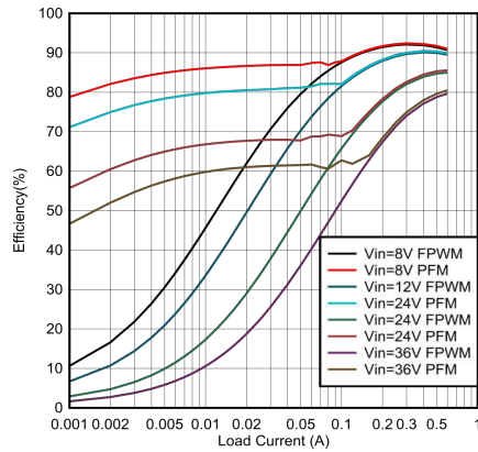
图 6-1. 3.3-V Efficiency Versus Load Current
