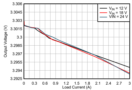
LMR66430MC3 V_{OUT} = 3.3V 2.2MHz (自动) 修复
