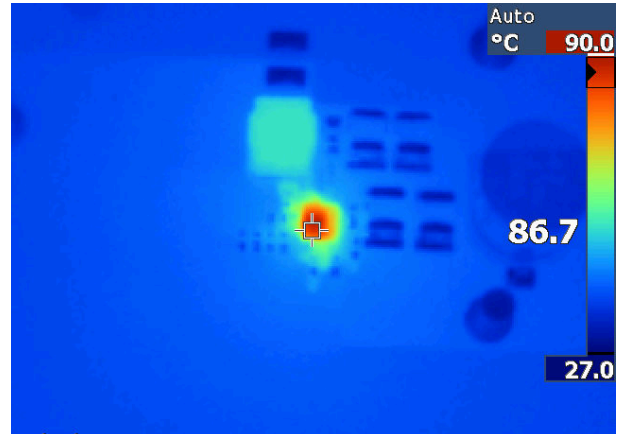
LMR66430MC3 V_{OUT} = 3.3V 12V_{IN} , 3A, 2.2MHz 修复
