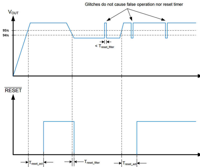
图 8-3. RESET Timing Behavior
