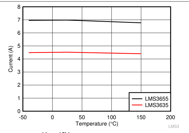
图 7-4. Low-Side/Valley Current Limit for LMS36x5-Q1
