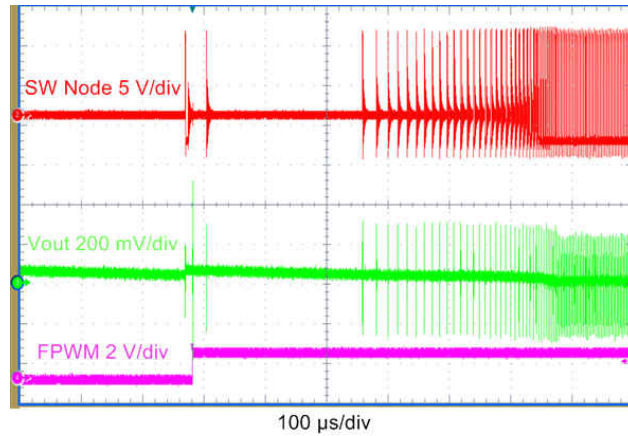
图 9-29. Mode Change Transient AUTO to FPWM mode
