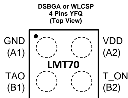
Pin Functions
