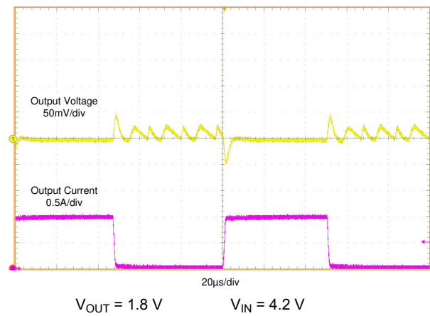
图 8-8. Load Transient In AUTO Mode
