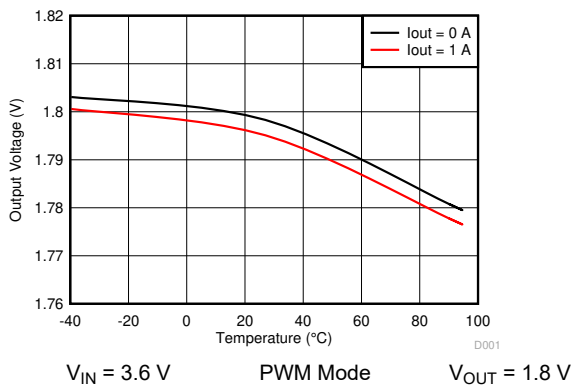
图 6-1. Typical Output Voltage vs Temperature
