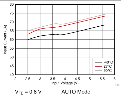
图 6-5. Non-Switching Input Current in AUTO Mode
