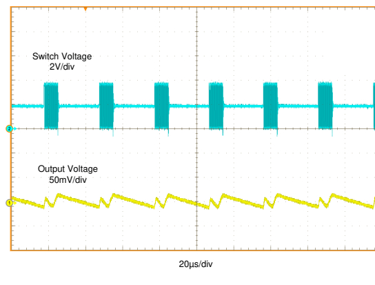
图 7-8. Typical PFM Mode Waveforms: V_{IN} = 3.6\text{ V} , V_{OUT} = 1.8\text{ V} , I_{OUT} = 10\text{ mA}
