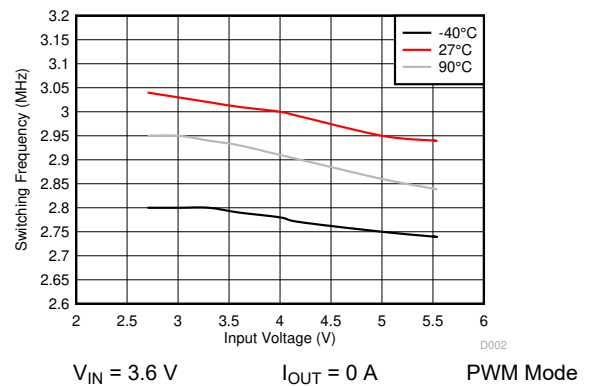
图 6-2. Switching Frequency in PWM Mode
