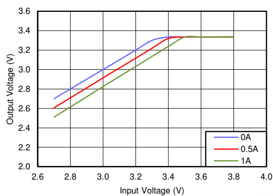
图 7-6. Typical Dropout Behavior, V_{OUT} = 3.3\text{ V}
