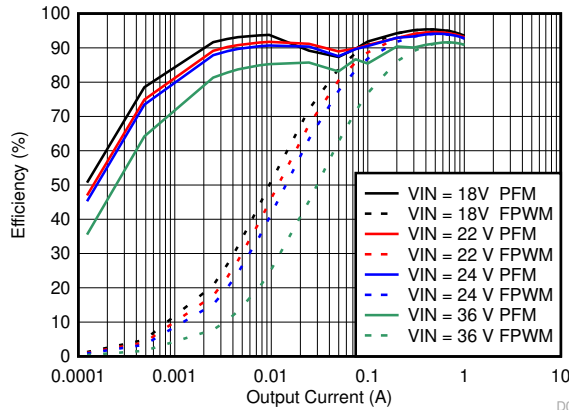
图 8-24. Efficiency
