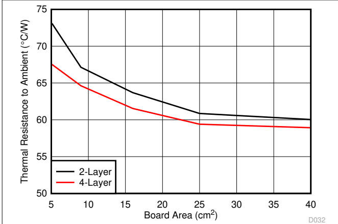
图 6-9. Package Thermal Resistance vs Board Copper Area, No Air Flow
