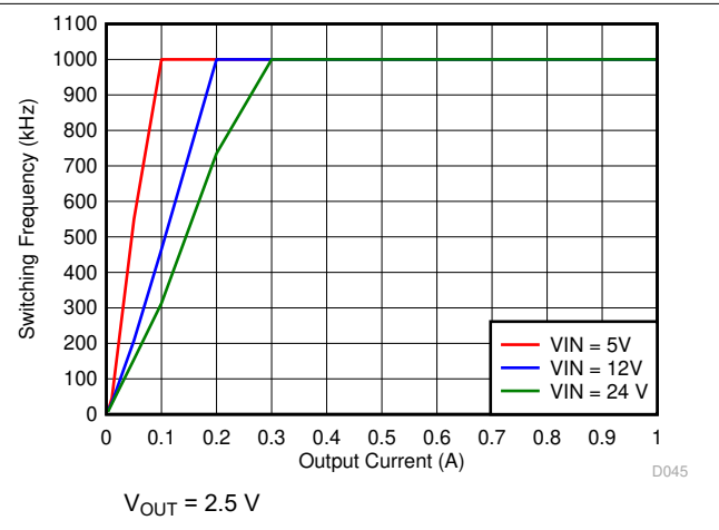
图 6-24. Auto PFM Mode Switching Frequency vs Output Current
