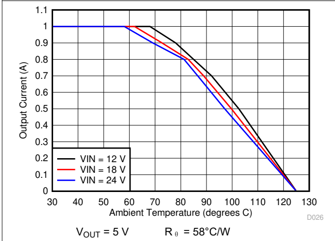
图 6-21. Ambient Temperature vs Output Current
