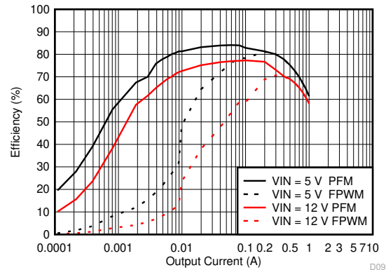
MODE = Low for Auto PFM Mode 1.2-V Adjustable Output MODE = High for FPWM Mode
