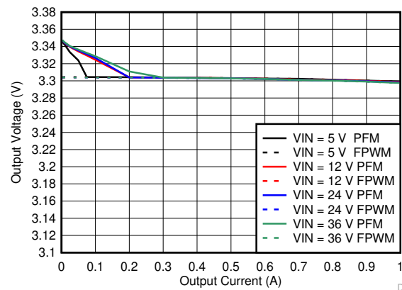
图 8-45. Line and Load Regulation for V_{OUT} = 3.3\text{ V}
