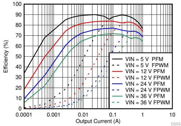
图 8-30. Efficiency
