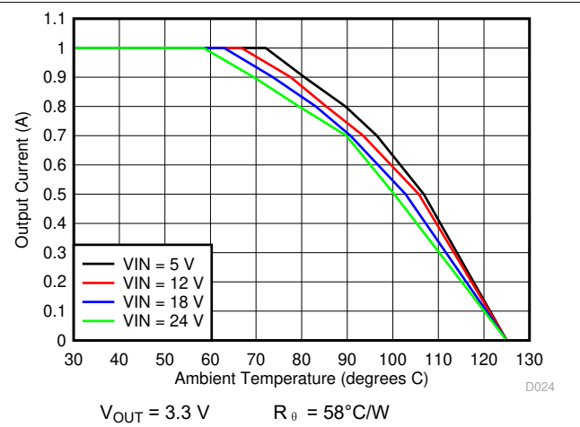
图 6-20. Ambient Temperature vs Output Current
