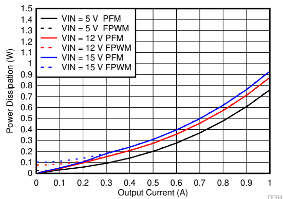
MODE = Low for Auto PFM Mode 1.8-V Adjustable Output MODE = High for FPWM Mode
