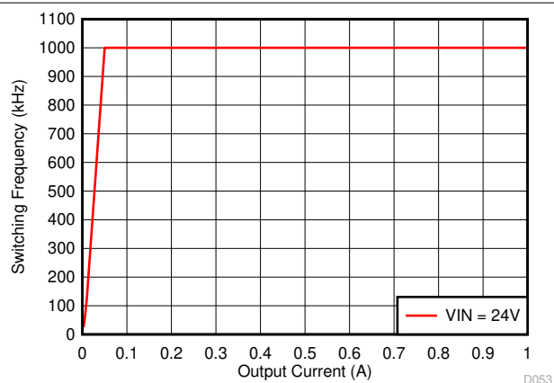
图 6-28. Auto PFM Mode Switching Frequency vs Output Current
