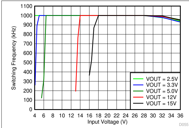
图 6-31. Switching Frequency vs Input Voltage for Adjustable Output Options at Full Load
