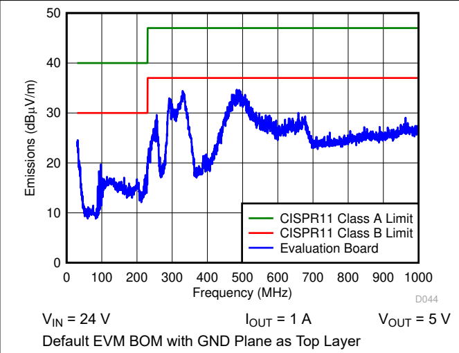
图 6-8. Radiated EMI
