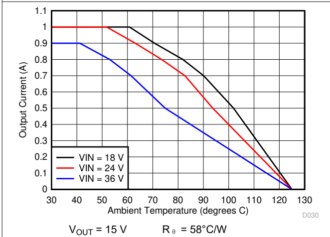
图 6-23. Ambient Temperature vs Output Current
