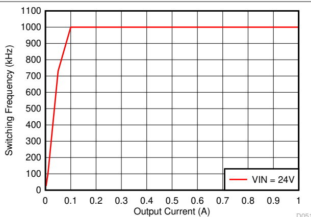
图 6-27. Auto PFM Mode Switching Frequency vs Output Current
