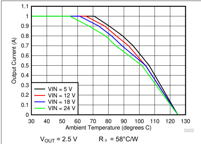
图 6-19. Ambient Temperature vs Output Current
