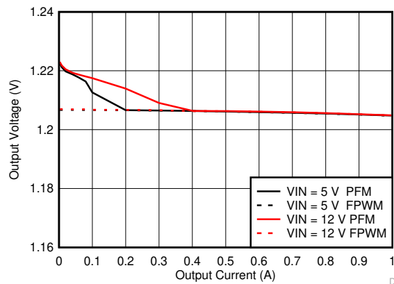
图 8-39. Line and Load Regulation for V_{OUT} = 1.2\text{ V}
