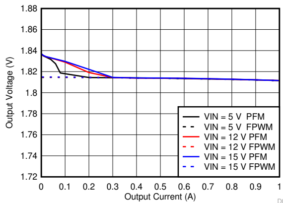
图 8-38. Line and Load Regulation for V_{OUT} = 1.8\text{ V}
