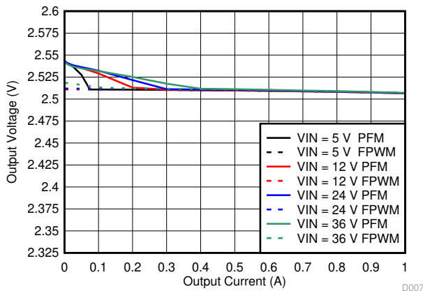
图 8-34. Line and Load Regulation
