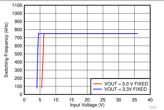
图 6-32. Switching Frequency vs Input Voltage for Fixed Output Options at Full Load
