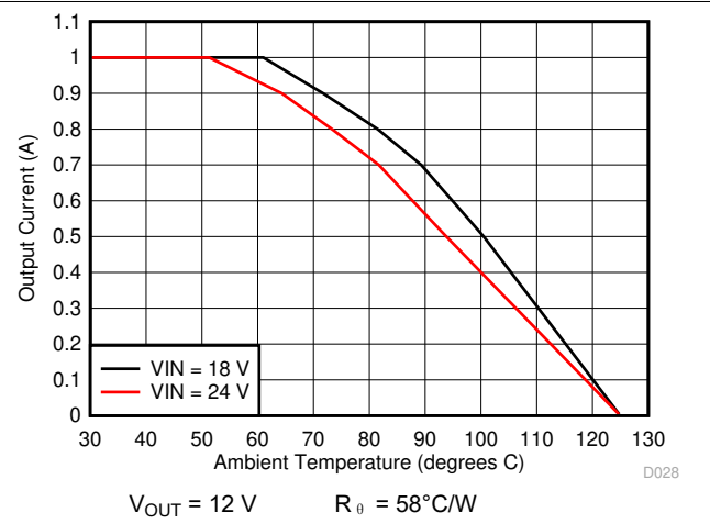
图 6-22. Ambient Temperature vs Output Current
