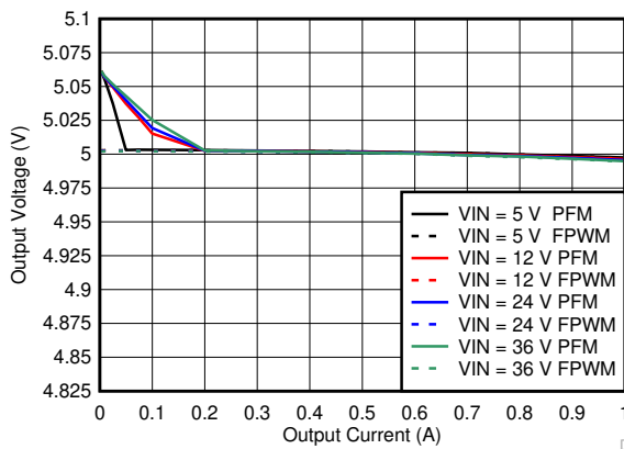
图 8-44. Line and Load Regulation for V_{OUT} = 5\text{ V}
