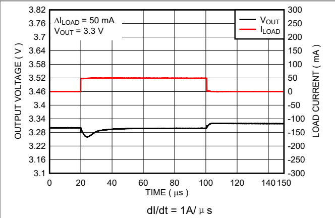
图 7-4. Load Transient Response (New Chip)
