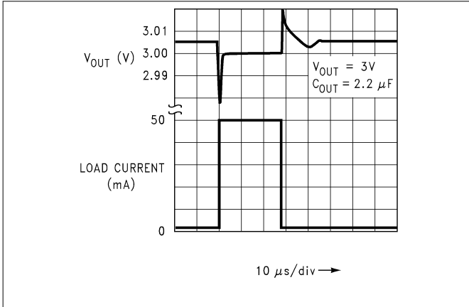
图 7-3. Load Transient Response (Legacy Chip)
