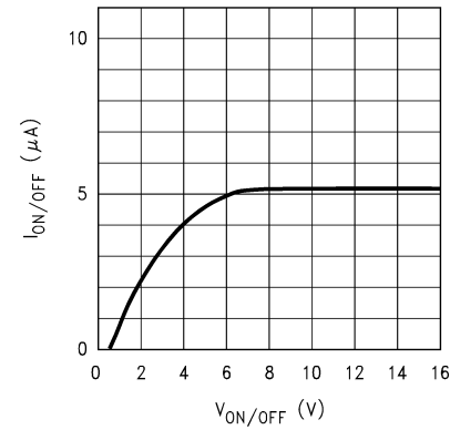
图 5-38. \text{ON}/\overline{\text{OFF}} Pin Current vs V_{\text{ON/OFF}} (Legacy Chip)
