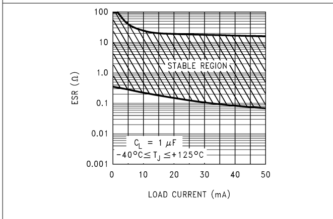
图 5-41. 1\mu\text{F} ESR Range vs I_{\text{OUT}} (Legacy Chip)
