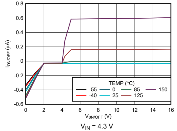
图 5-40. \text{ON}/\overline{\text{OFF}} Pin Current vs V_{\text{ON/OFF}} (New Chip)
