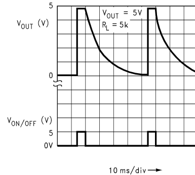
图 5-34. Turn-On Waveform (Legacy Chip)
