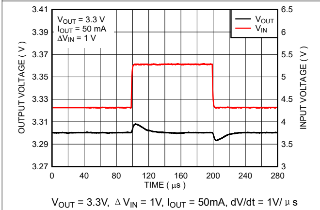
图 7-5. Line Transient Response (New Chip)
