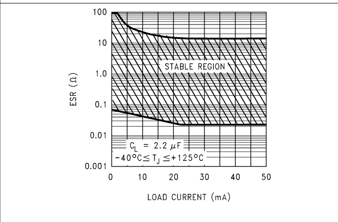
图 5-42. 2.2\mu\text{F} ESR Range vs I_{\text{OUT}} (Legacy Chip)
