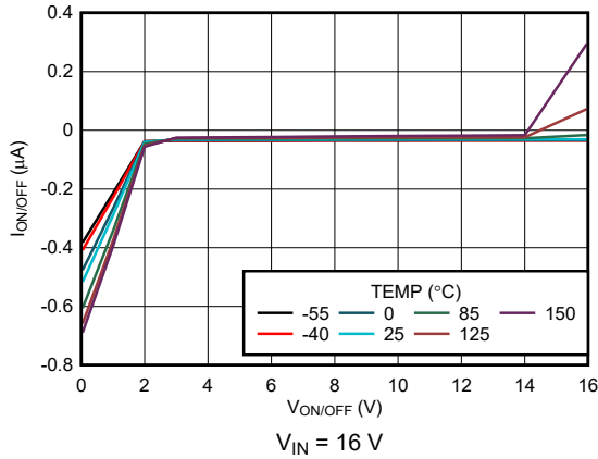
图 5-39. \text{ON}/\overline{\text{OFF}} Pin Current vs V_{\text{ON/OFF}} (New Chip)
