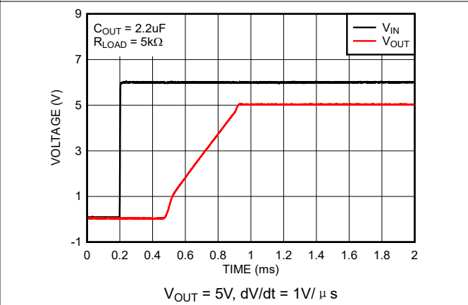
图 7-6. Start-Up (New Chip)
