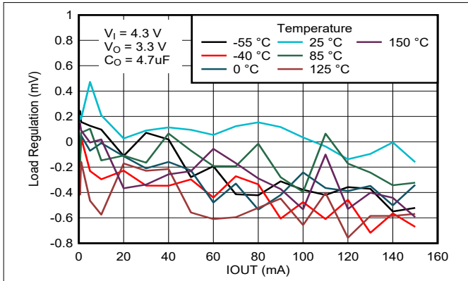
图 6-7. Output Regulation vs Load Current for New Chip
