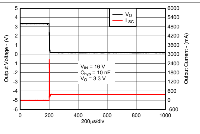
图 6-12. Short-Circuit Current vs Time for New Chip
