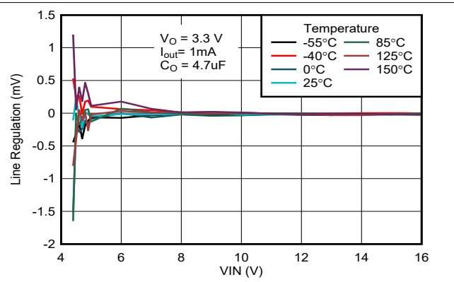
图 6-8. Output Regulation vs Input Voltage for New Chip
