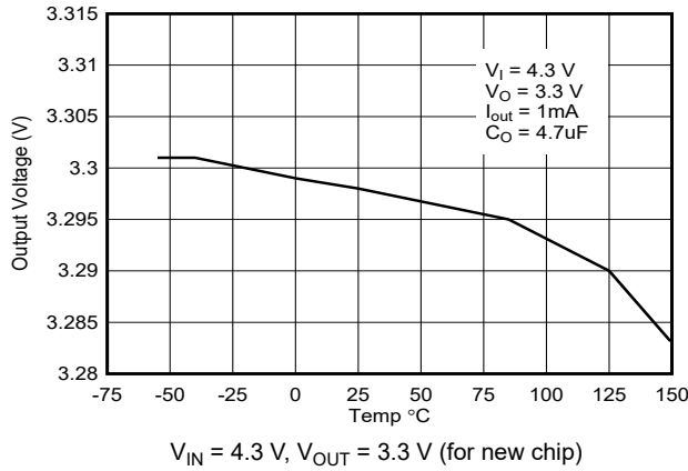
图 6-3. Output Voltage vs Temperature for New Chip
