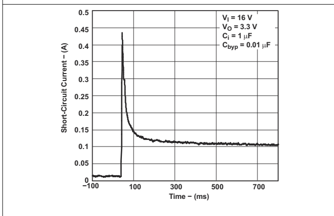
图 6-11. Short-Circuit Current vs Time for Legacy Chip
