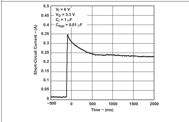
图 6-9. Short-Circuit Current vs Time for Legacy Chip
