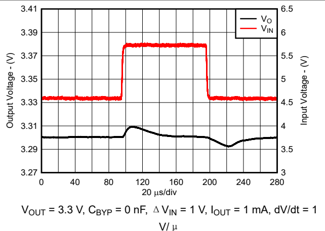
图 8-14. Line Transient Response for New Chip
