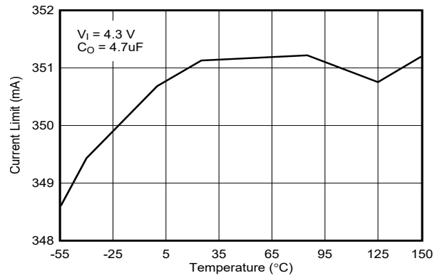
图 6-32. Short-Circuit Current vs Temperature for New Chip
