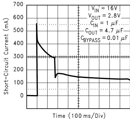
图 5-3. Short-Circuit Current for Legacy Chip
