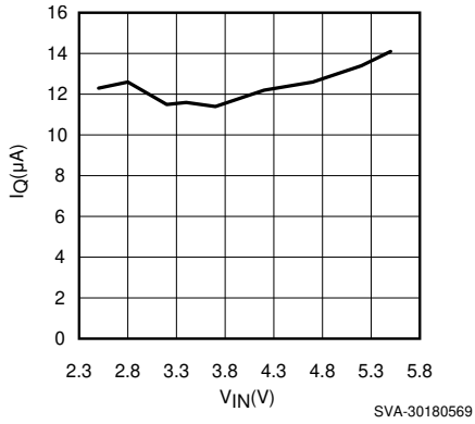
图 5-1. Quiescent Current vs Input Voltage
