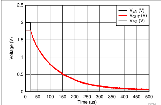
图 6-39. LP5912-1.8 V_{OUT} vs V_{EN(OFF)}
