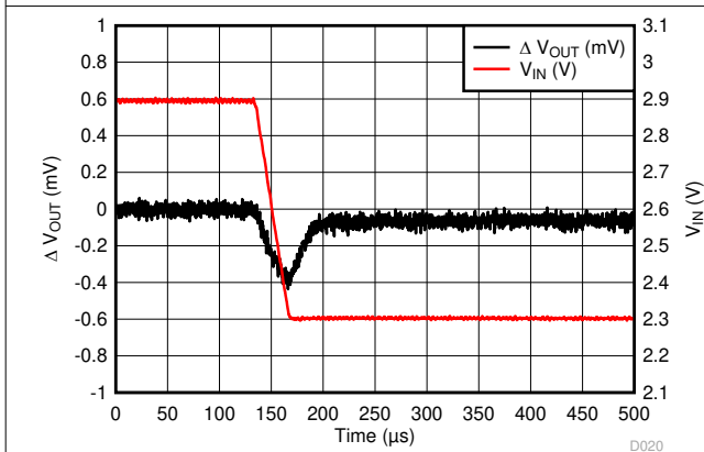
图 6-27. LP5912-0.9 Line Transient
