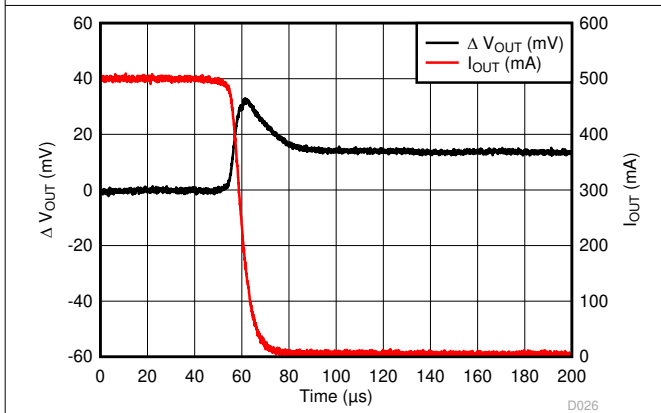
图 6-33. LP5912-0.9 Load Transient Response
