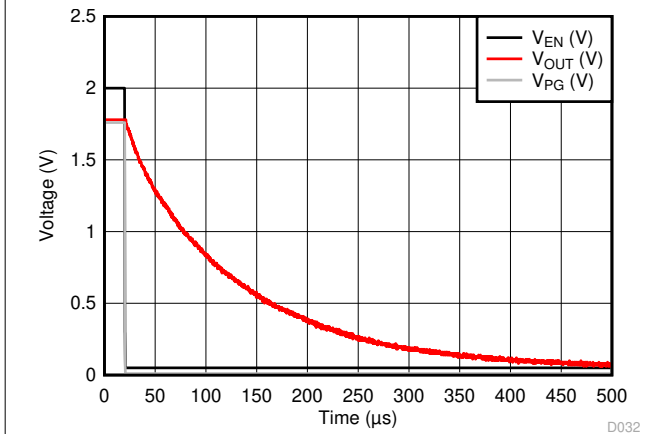
图 6-39. LP5912-1.8 V_{OUT} vs V_{EN(OFF)}
