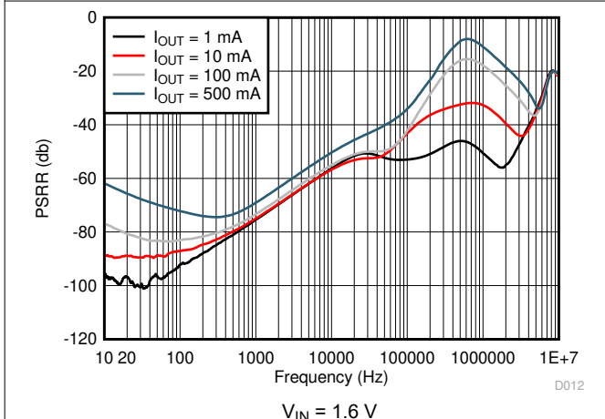
图 6-21. LP5912-0.9 PSRR vs Frequency
