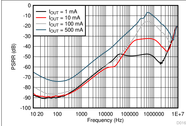
图 6-25. LP5912-3.3 PSRR vs Frequency
