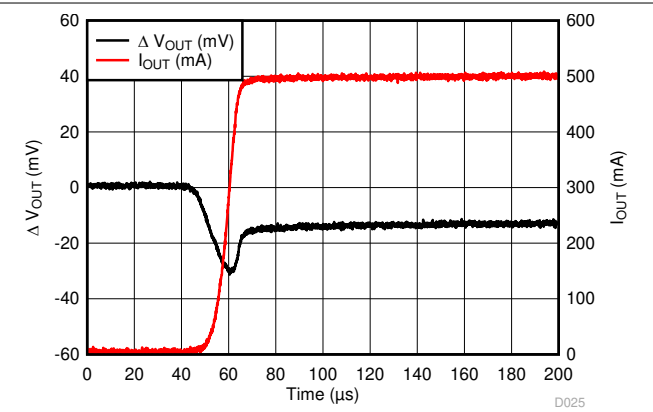
图 6-32. LP5912-0.9 Load Transient Response
