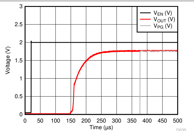
图 6-40. LP5912-1.8 V_{OUT} vs V_{EN(ON)}
