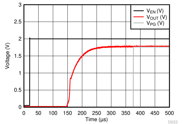
图 6-38. LP5912-1.8 V_{OUT} vs V_{EN(ON)}
