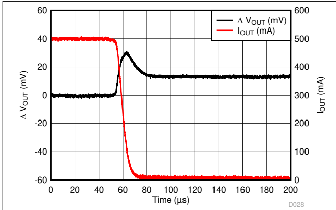
图 6-37. LP5912-3.3 Load Transient Response
