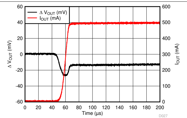
图 6-34. LP5912-1.8 Load Transient Response
