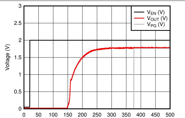
图 6-38. LP5912-1.8 V_{OUT} vs V_{EN(ON)}
