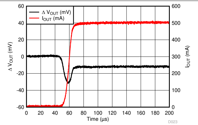
图 6-32. LP5912-0.9 Load Transient Response
