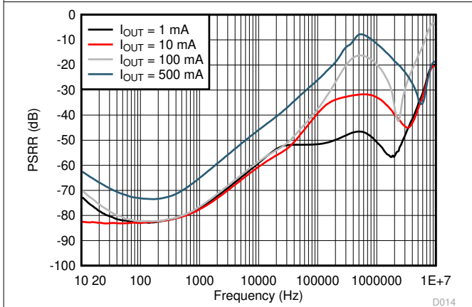
图 6-21. LP5912-0.9 PSRR vs Frequency
