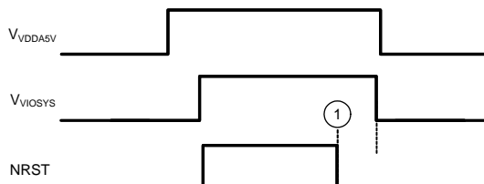
Figure 12. The External Power Control System De-asserts NRST
