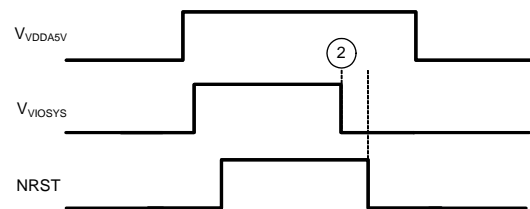
Figure 13. NRST Stays HIGH While V_{VIO SYS} Transition from HIGH to LOW Happens (Marked as '2')
