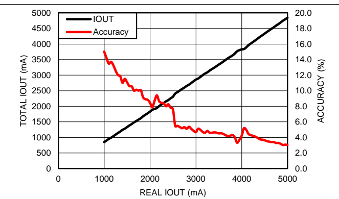
Figure 38. Load Current Measured by LP8754 vs Real Load Current, 3 Phases Active
