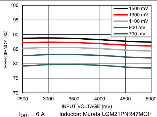
Figure 30. Efficiency vs Input Voltage in PWM Mode
