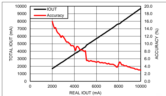
Figure 37. Load Current Measured by LP8754 vs Real Load Current, 6 Phases Active
