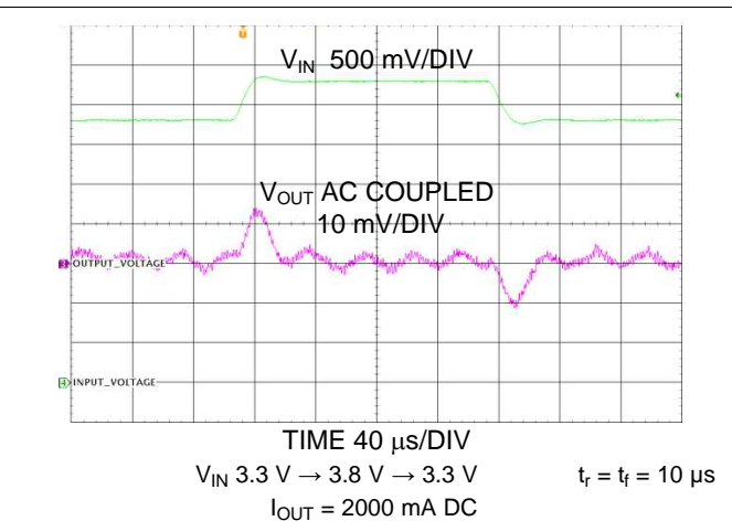
Figure 42. Transient Line Response
