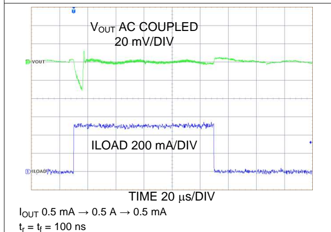
Figure 41. Transient Load Step Response, AUTO Mode
