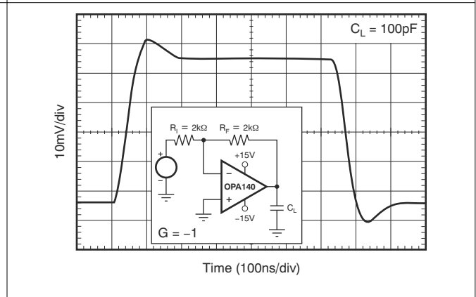
图 6-28. Small-Signal Step Response (100 mV)
