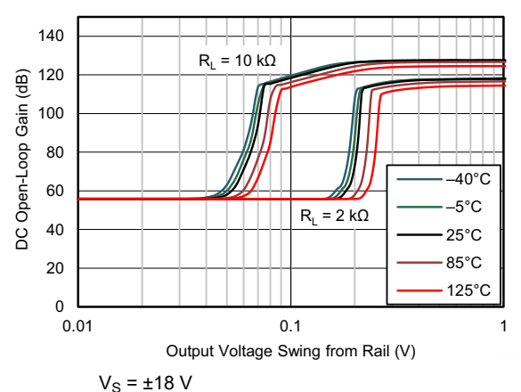
图 6-24. Open-Loop Gain vs Output Voltage Swing to Supply
