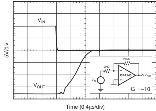
图 6-24. Negative Overload Recovery
