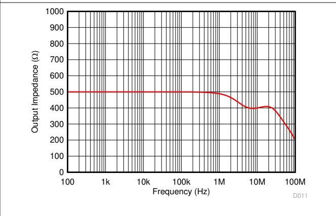
图 7-12. Open Loop Output Impedance vs Frequency
