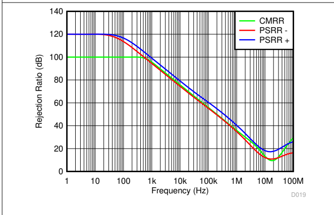
图 7-11. Rejection Ratio vs frequency
