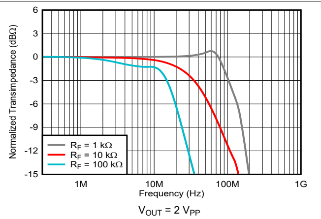
图 6-4. Large-Signal Frequency Response vs Gain
