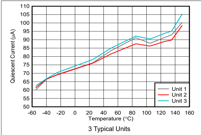
图 6-19. Quiescent Current (Amplifiers Disabled) vs Ambient Temperature
