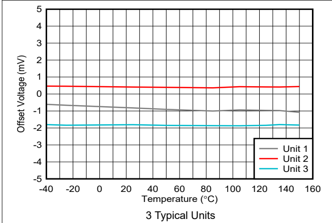
图 6-21. Offset Voltage vs Ambient Temperature
