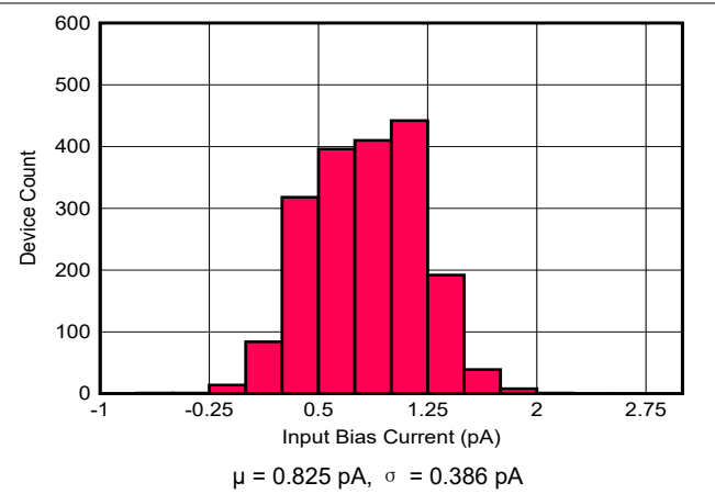
图 6-34. Input Bias Current Distribution – Channel B
