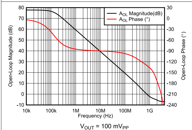
图 6-5. Open-Loop Magnitude and Phase vs Frequency
