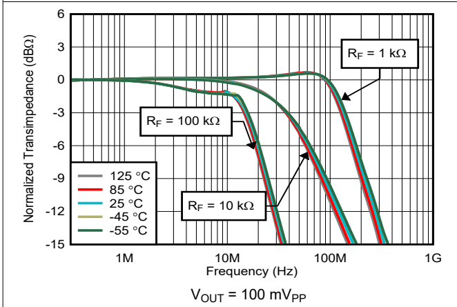
图 6-3. Small-Signal Frequency Response vs Ambient Temperature
