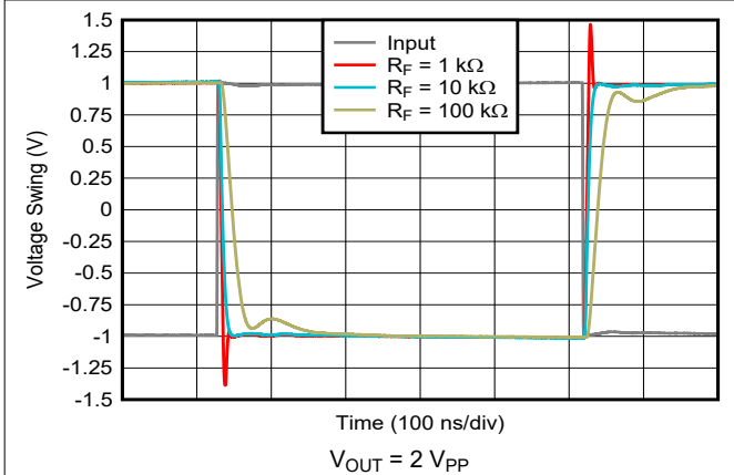
图 6-11. Large-Signal Transient Response
