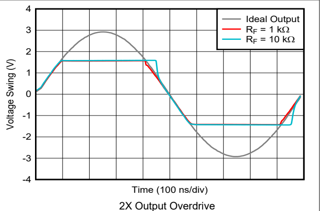
图 6-12. Output Overload Reponse – Low Gain Settings
