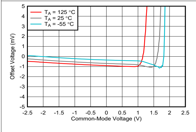
图 6-23. Offset Voltage vs Input Common-Mode Voltage vs Ambient Temperature
