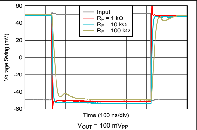
图 6-10. Small-Signal Transient Response
