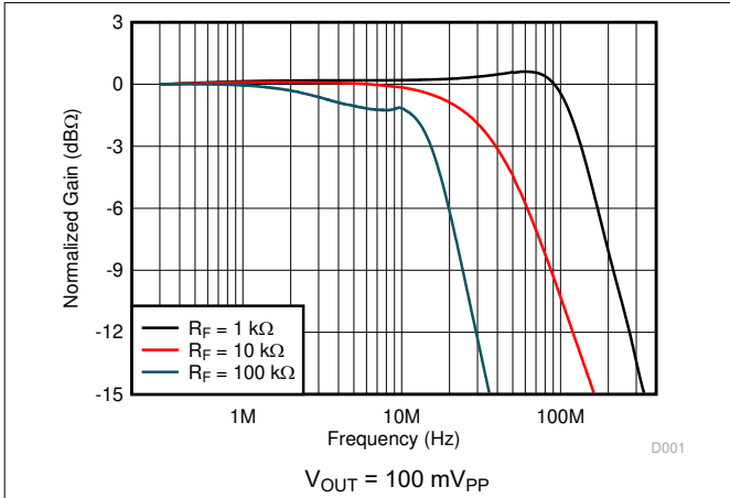
图 6-1. Small-Signal Frequency Response vs Gain
