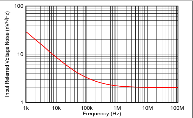
图 6-8. Voltage Noise Density vs Frequency
