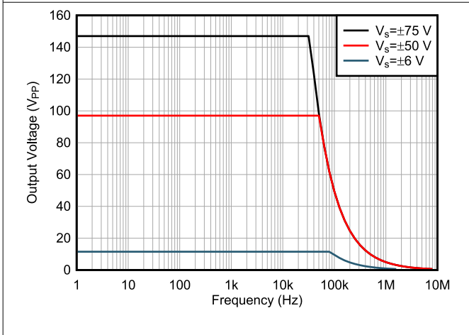
图 6-29. Maximum Output Voltage vs Frequency
