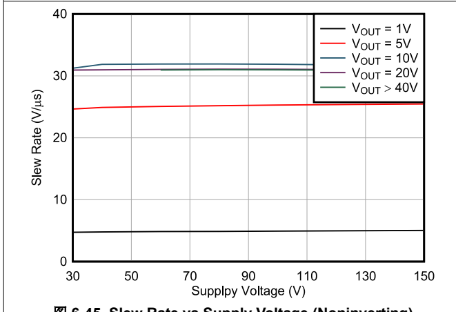
图 6-45. Slew Rate vs Supply Voltage (Noninverting)
