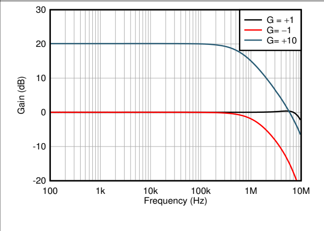
图 6-28. Closed-Loop Gain vs Frequency
