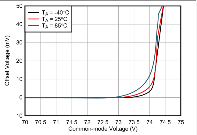
图 6-8. Offset Voltage vs Common-Mode Voltage (High V_{CM} )
