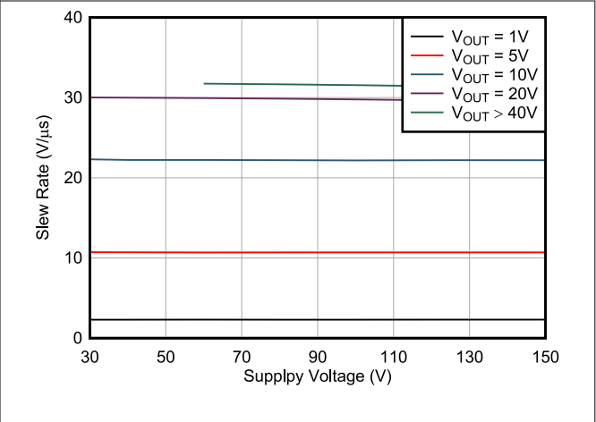
图 6-44. Slew Rate vs Supply Voltage (Inverting)
