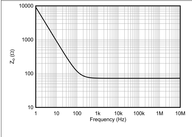
图 6-27. Open-Loop Output Impedance vs Frequency
