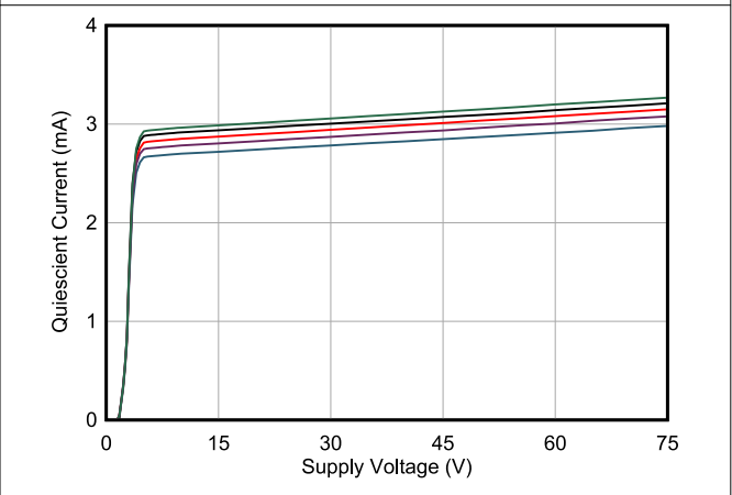
图 6-54. Quiescent Current vs Supply Voltage
