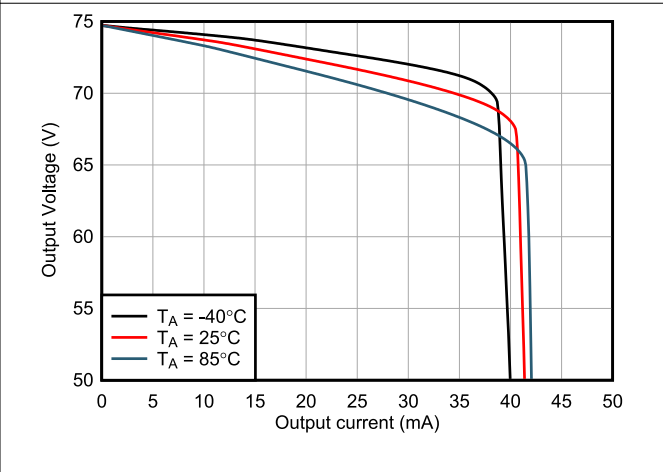
图 6-30. Positive Output Voltage vs Output Current
