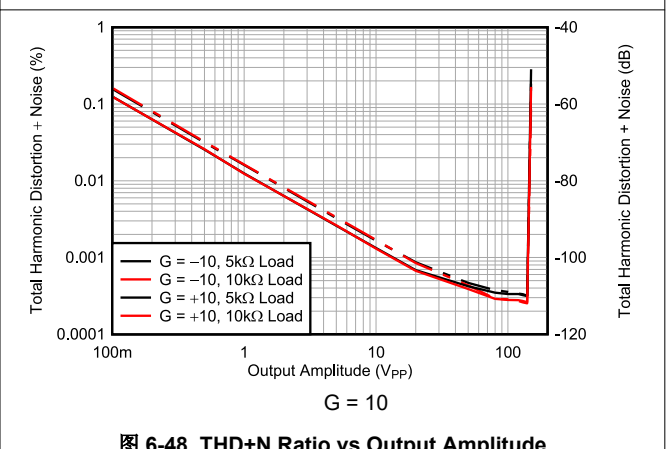
图 6-48. THD+N Ratio vs Output Amplitude
