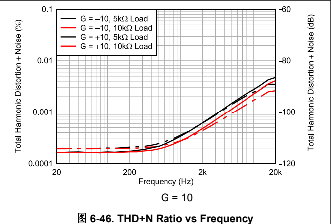
图 6-46. THD+N Ratio vs Frequency
