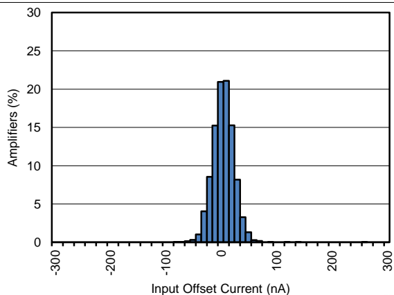
图 45. Input Offset Current Distribution
