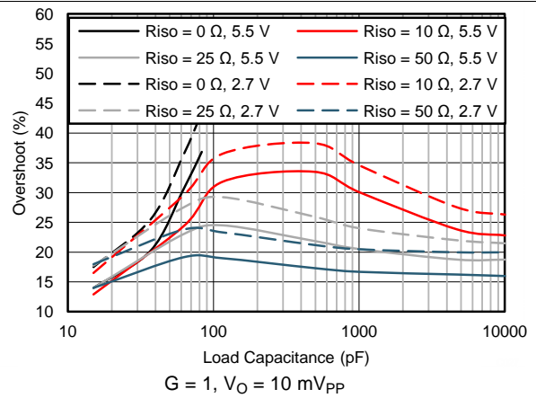
图 15. Overshoot vs Capacitive Load, G = 1
