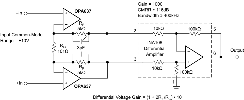
图 7-2. High Speed Instrumentation Amplifier, Gain = 1000
