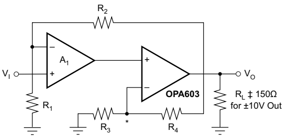
图 7-3. Composite Amplifier for Wide Bandwidth
