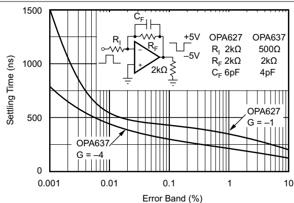
图 5-25. Settling Time vs Error Band
