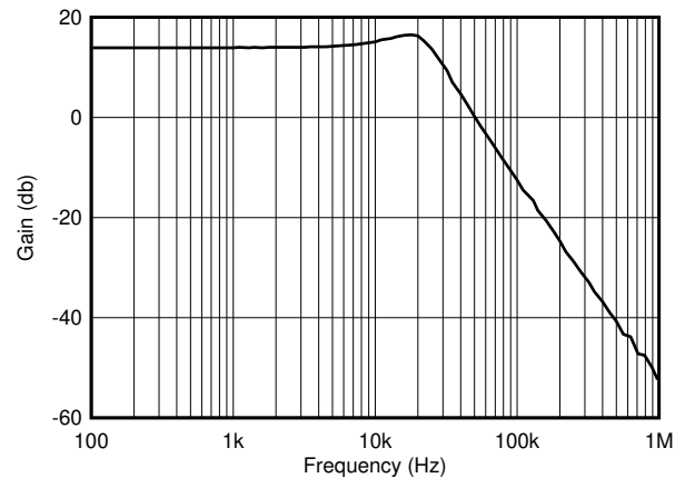
图 7-8. OPA627 2nd Order 25kHz, Chebyshev, Low-Pass Filter
