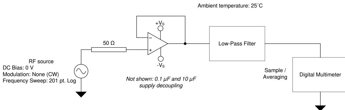
图 6-9. EMIRR IN+ Test Configuration Schematic
