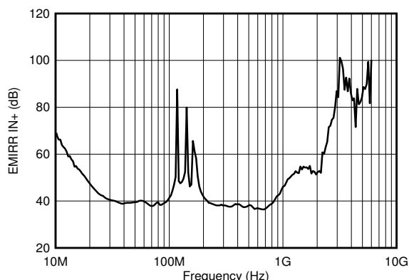
图 6-8. OPA627 (SOIC packages) EMIRR IN+ vs Frequency
