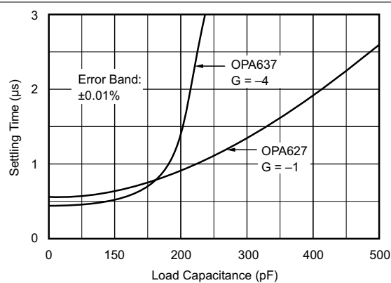
图 5-26. Settling Time vs Load Capacitance
