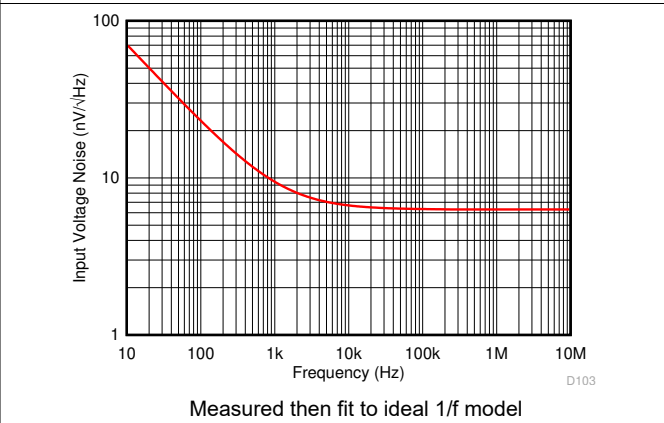
图 6-47. Input Voltage Noise Density vs Frequency
