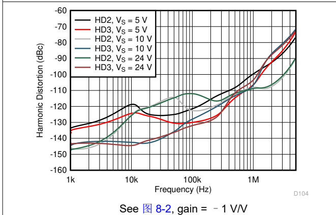
图 6-46. Harmonic Distortion vs Frequency vs Supply Voltage
