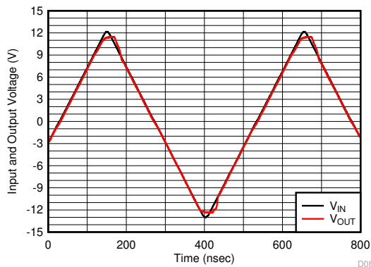
图 6-27. Large-Signal Transient Response
