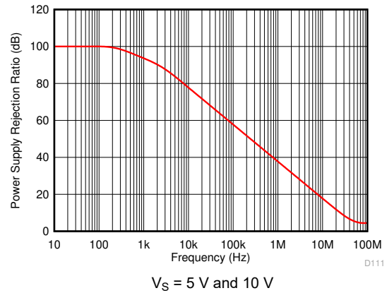
图 6-51. Power Supply Rejection Ratio vs Frequency
