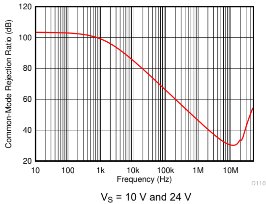
图 6-50. Common-Mode Rejection Ratio vs Frequency
