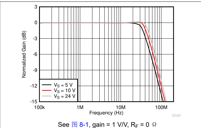
图 6-43. Large-Signal Response vs Supply Voltage
