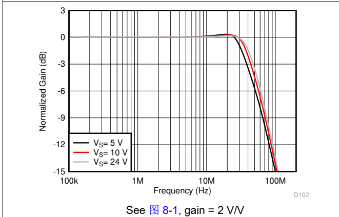
图 6-44. Large-Signal Response vs Supply Voltage
