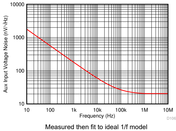
图 6-48. Auxiliary Input Stage Voltage Noise Density vs Frequency
