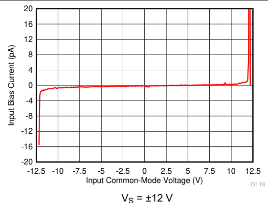
图 6-53. Input Bias Current vs Input Common-Mode Voltage
