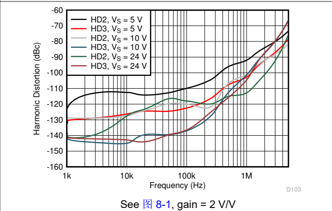
图 6-45. Harmonic Distortion vs Frequency vs Supply Voltage
