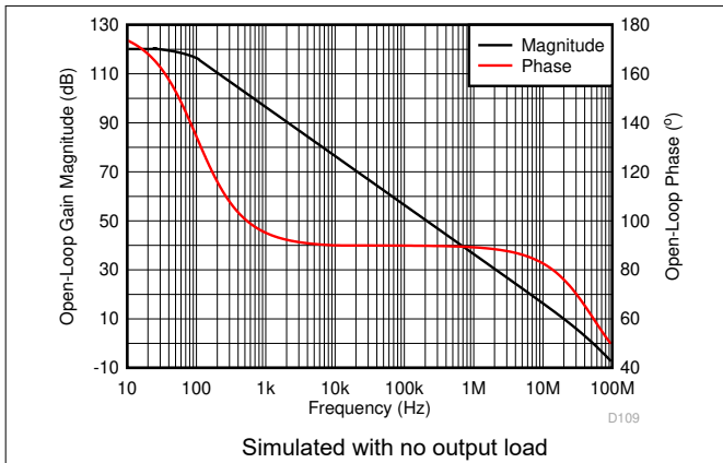
图 6-42. Open-Loop Gain and Phase vs Frequency
