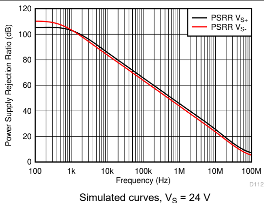
图 6-52. Power Supply Rejection Ratio vs Frequency
