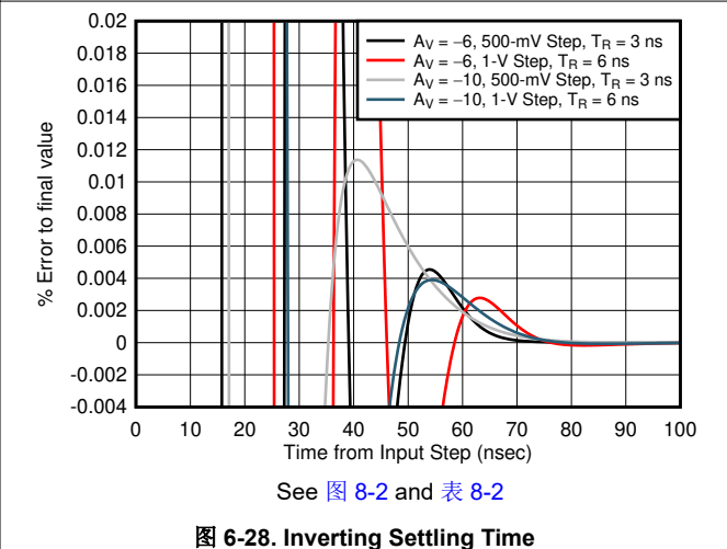
图 6-28. Inverting Settling Time
