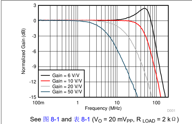
图 6-1. Noninverting Small-Signal Frequency Response vs Gain
