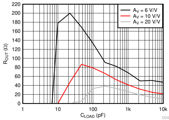
图 6-49. Output Resistor vs C_{LOAD}
