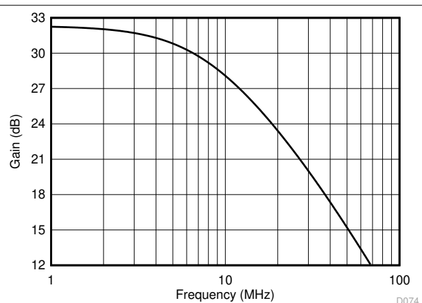
图 8-6. Differential Small-Signal Frequency Response
