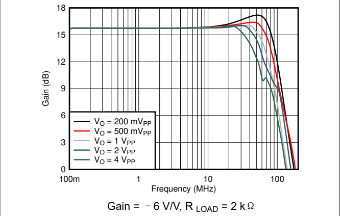
图 6-4. Inverting Large-Signal Bandwidth vs V_{OPP}
