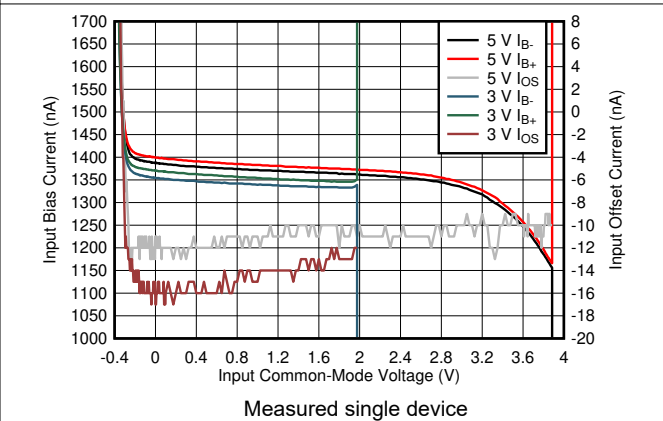
图 6-60. Input Bias and Offset Current vs V_{ICM}
