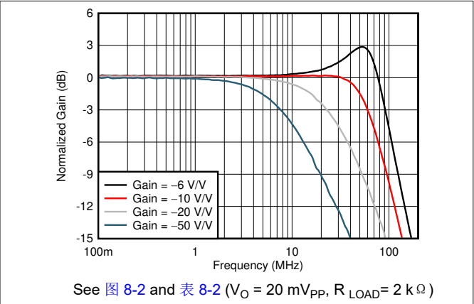
图 6-2. Inverting Small-Signal Frequency Response vs Gain
