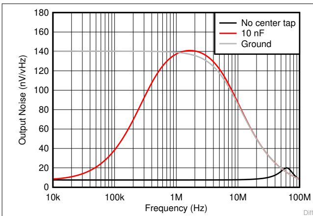
图 8-5. Common-Mode Output Noise for Differential I/O Design
