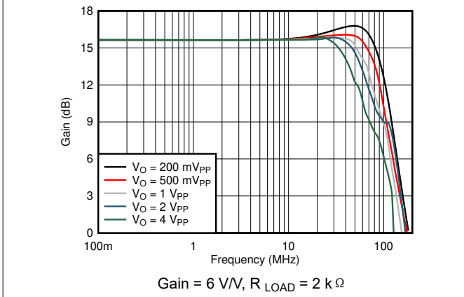
图 6-3. Noninverting Large-Signal Bandwidth vs V_{OPP}
