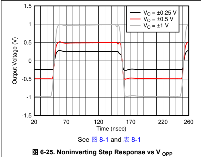
图 6-25. Noninverting Step Response vs V_{OPP}
