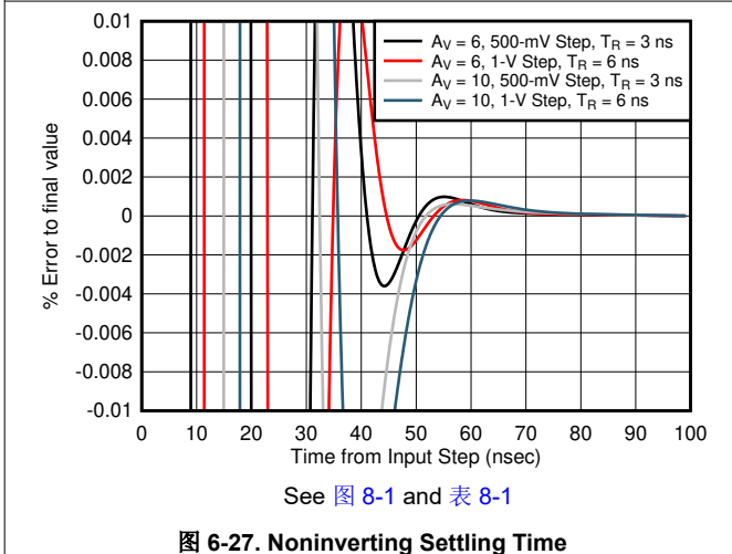
图 6-27. Noninverting Settling Time
