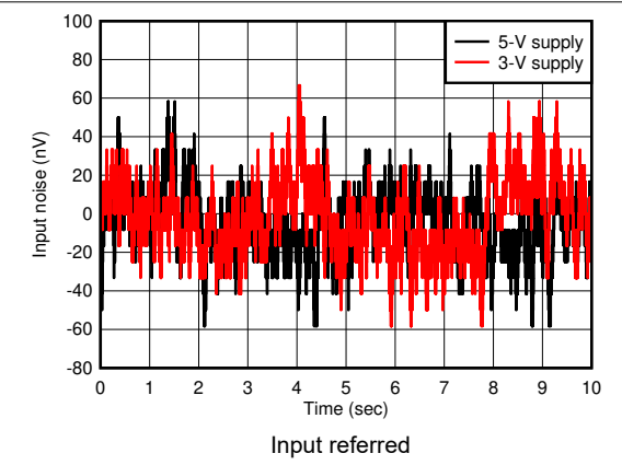
图 6-40. Low-Frequency Voltage Noise
