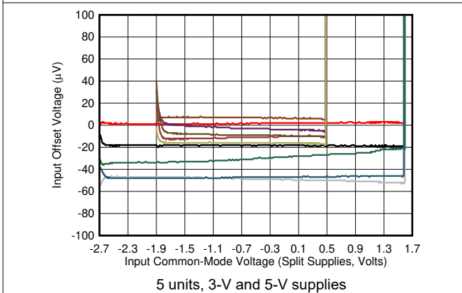
图 6-59. Input Offset Voltage vs Input Common-Mode Voltage
