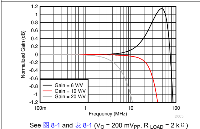
图 6-5. Noninverting Response Flatness vs Gain
