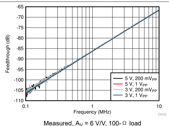
图 6-42. Disabled Isolation Noninverting Input to Output
