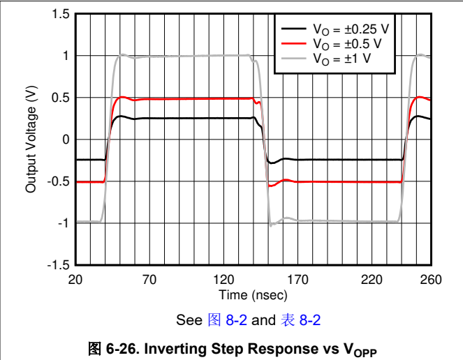
图 6-26. Inverting Step Response vs V_{OPP}
