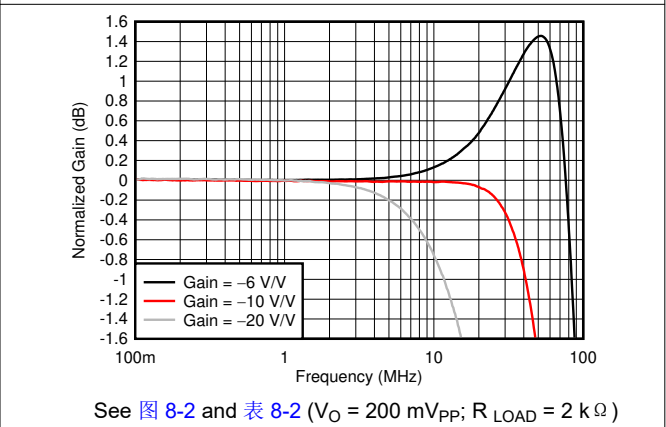
图 6-6. Inverting Response Flatness vs Gain
