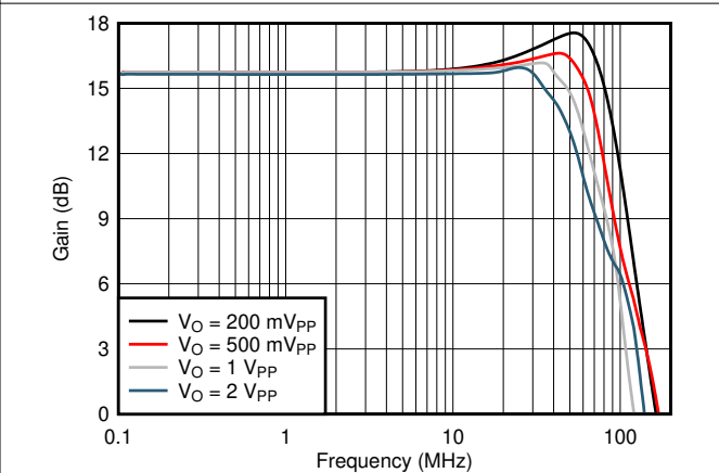
See 图 8-2 ( A_V = -6\text{ V/V} )
