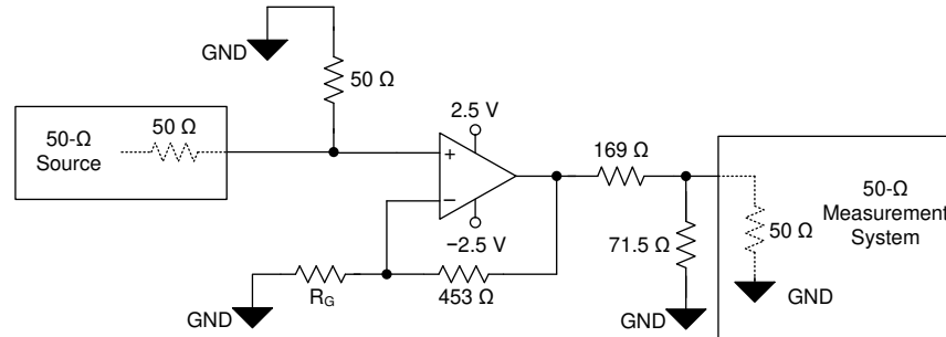
图 8-1. Noninverting Configuration
