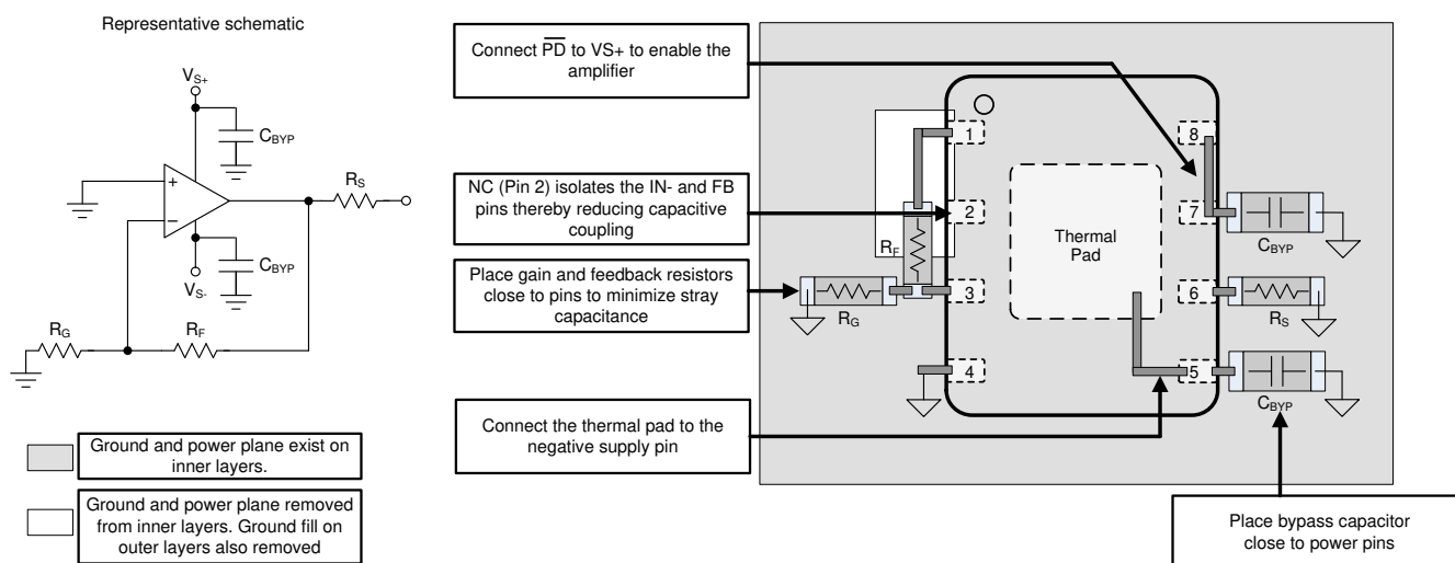
图 12-1. Layout Recommendation
