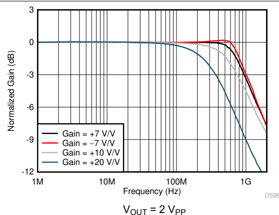
图 7-6. Large-Signal Frequency Response vs Gain
