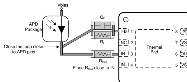
图 12-3. Improved TIA Layout
