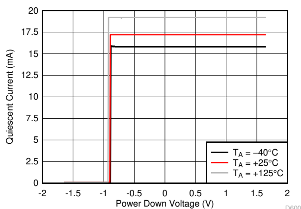
图 9-8. Switching Threshold (PD Pin Swept from High to Low)
