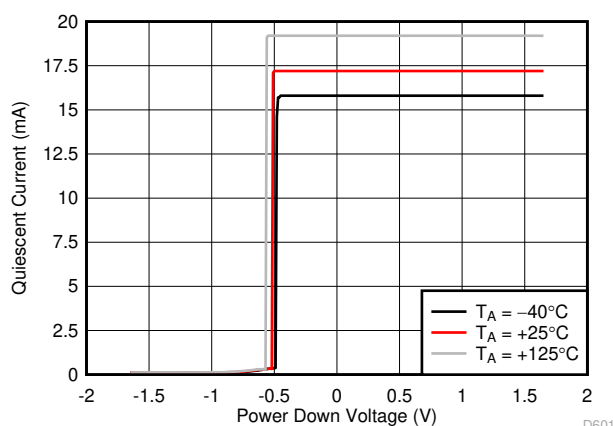
图 9-9. Switching Threshold (PD Pin Swept from Low to High)
