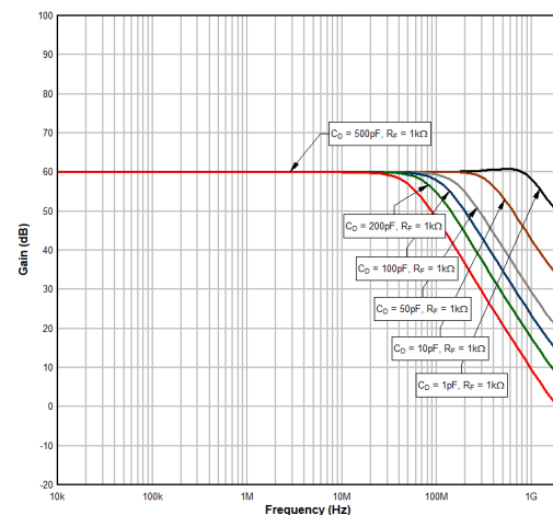
图 10-8. 1 Photodetector Input Characteristics TIA Frequency Response
