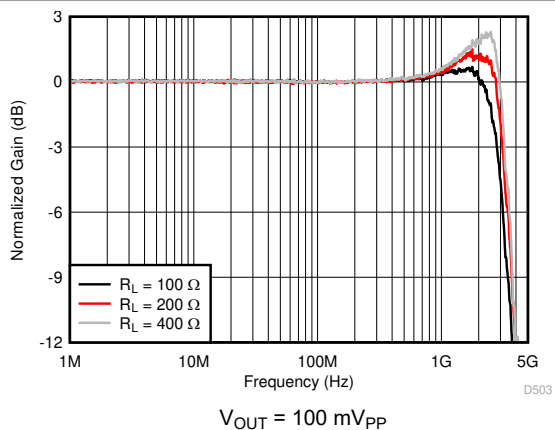
图 7-3. Small-Signal Frequency Response vs Output Load
