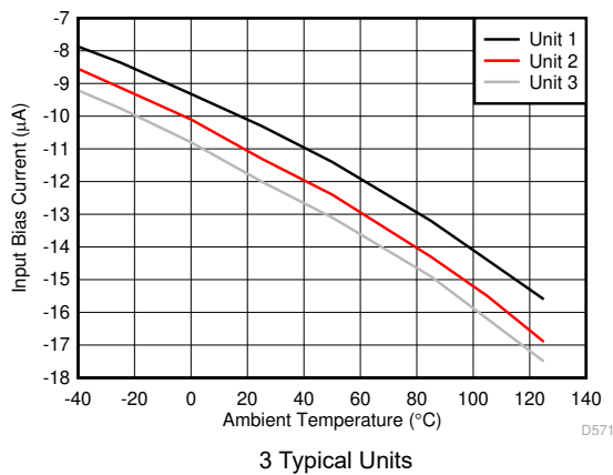
图 7-35. Input Bias Current vs Ambient Temperature
